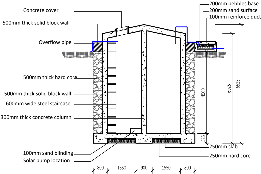
SECTION X-X
