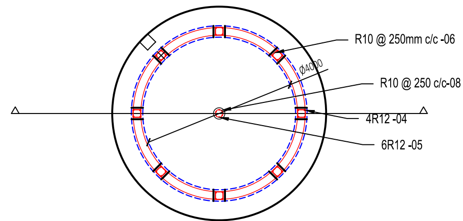
column layout
