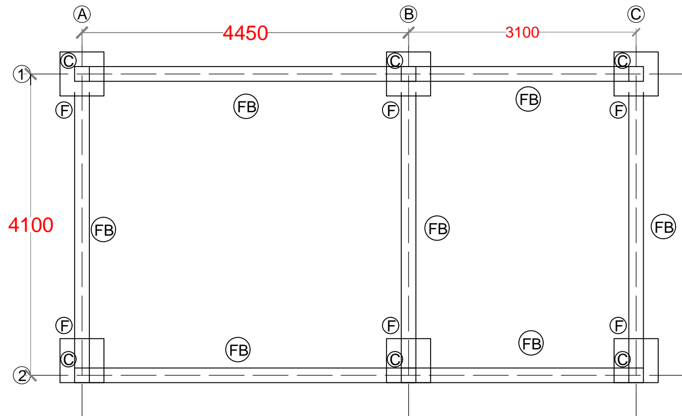
FOUNDATION PLAN
