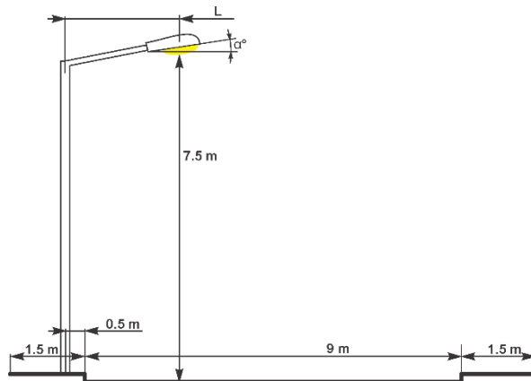
Sketch 2. 710m of Getapnya street
