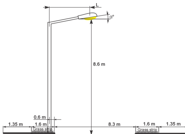
Sketch 4. Hanrapetutyany street
