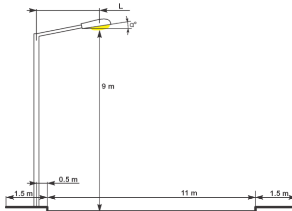
Sketch 7. Location of lighting poles on section of Virahayots road
