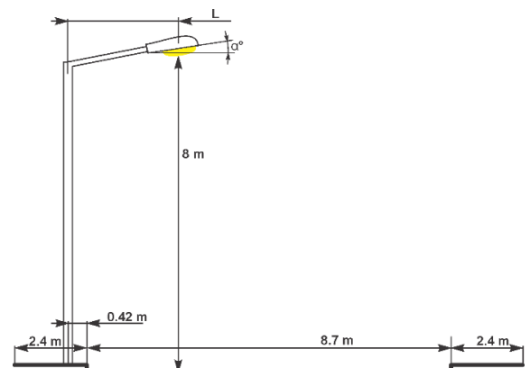
Sketch 5. Yerevanyany street
