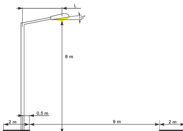
Sketch 1. Location of poles on section
