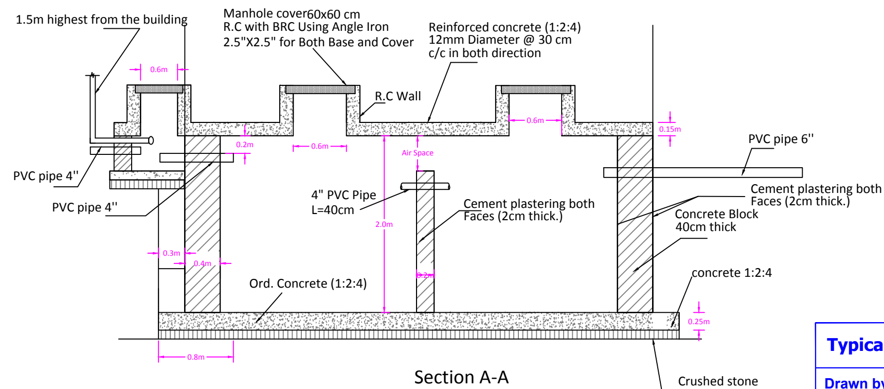
Standard Detail
