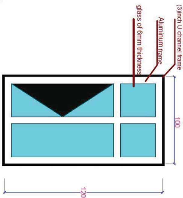
Aluminum Window
