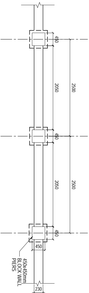
PERIMETER FENCE TYPICAL ELEVATION
