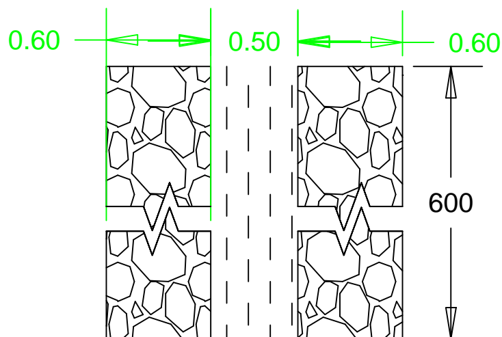
Plan detail -A -length= 600m
