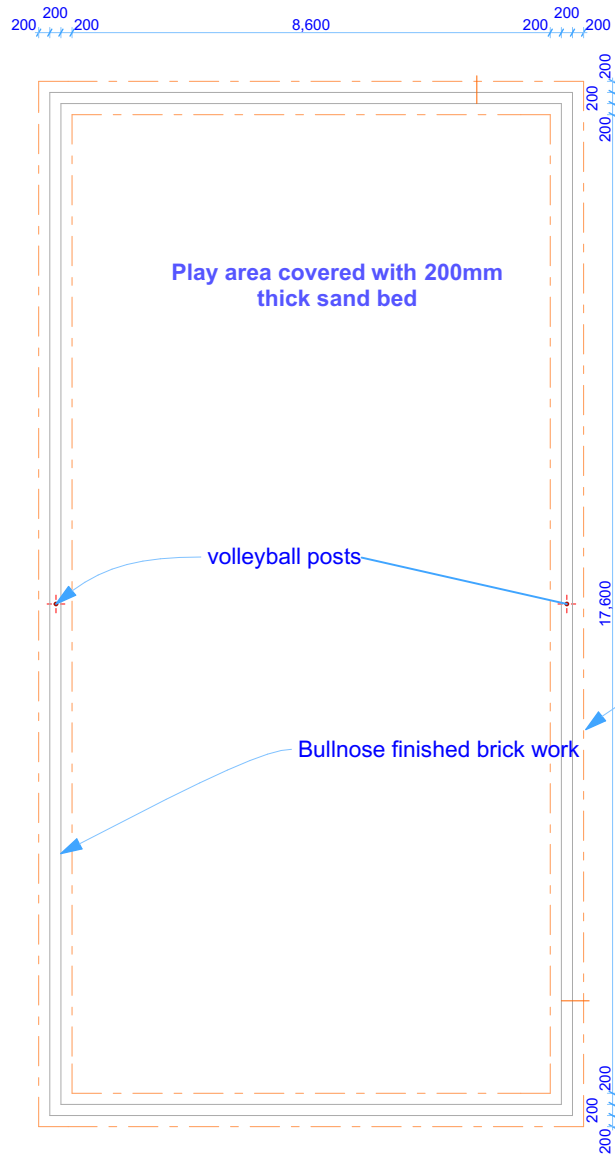
Volleyball court excavation & wall details
