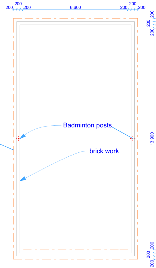
Badminton court excavation & wall details
