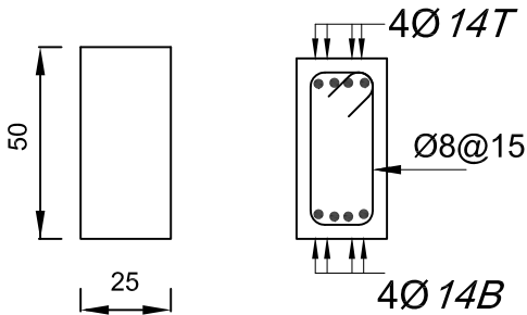
Beam B1 (1:25)
