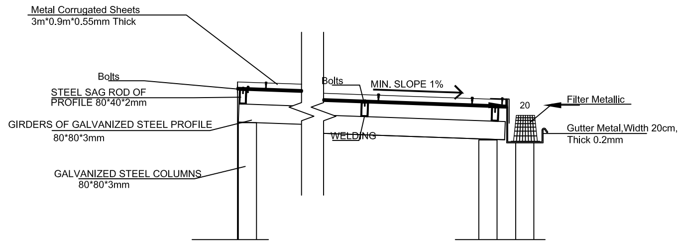
DETAIL 1
