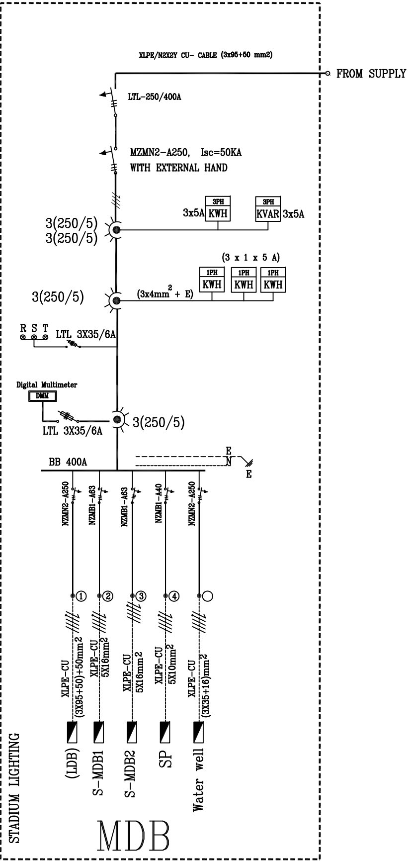
MDB SINGLE LINE DIAGRAM
