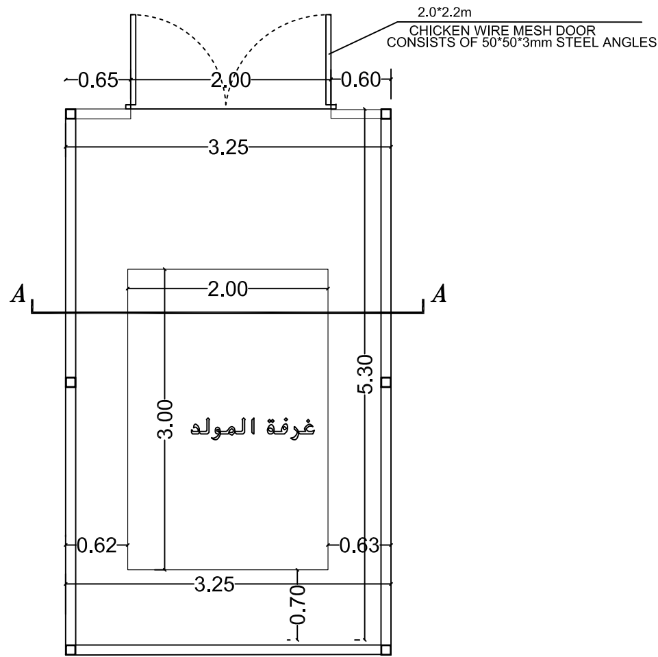
PLAN FOR GENERATOR SHED & FENCE SCALE 1 :50
