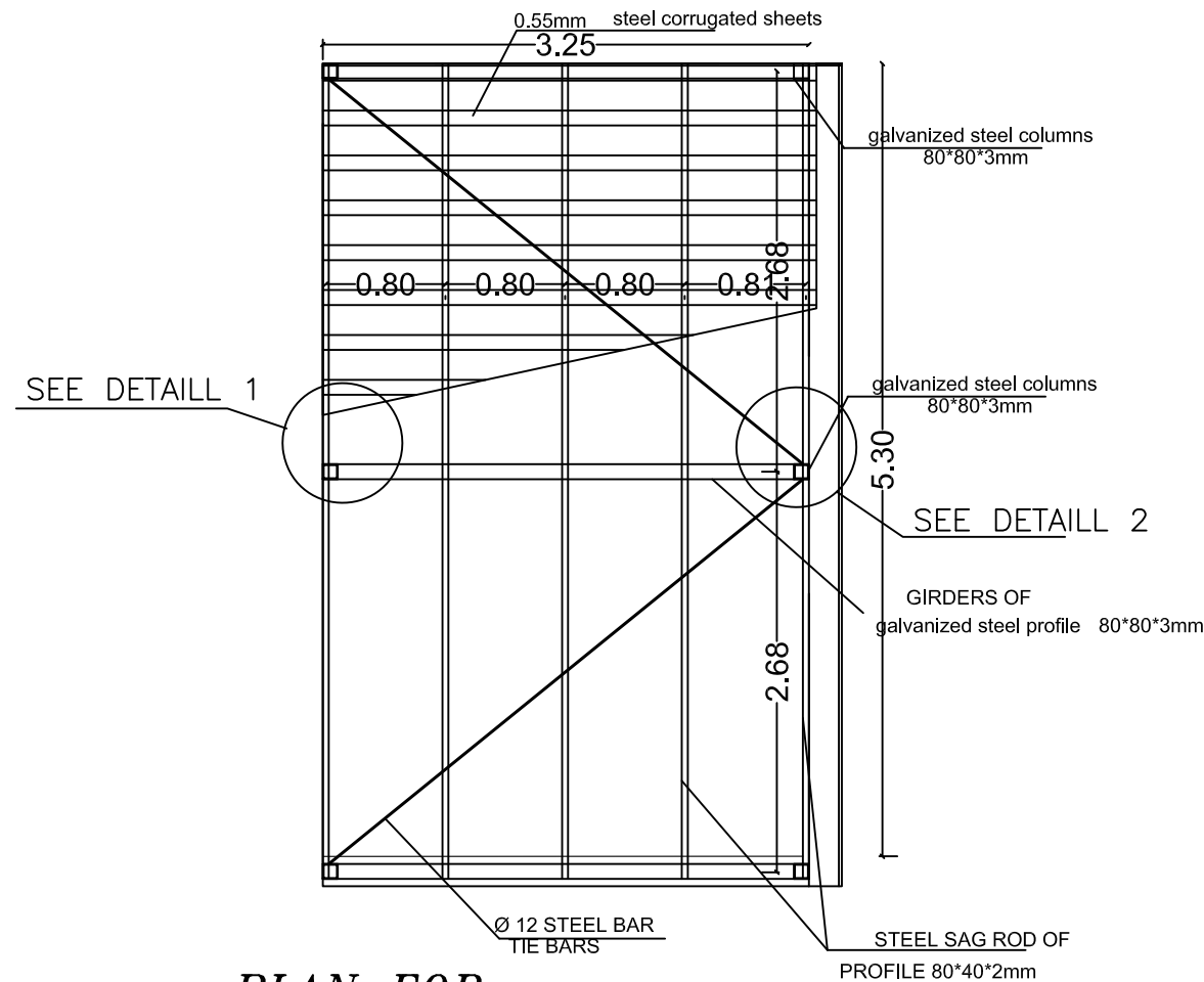
PLAN FOR GENERATOR SHED & FENCE SCALE 1 :50
