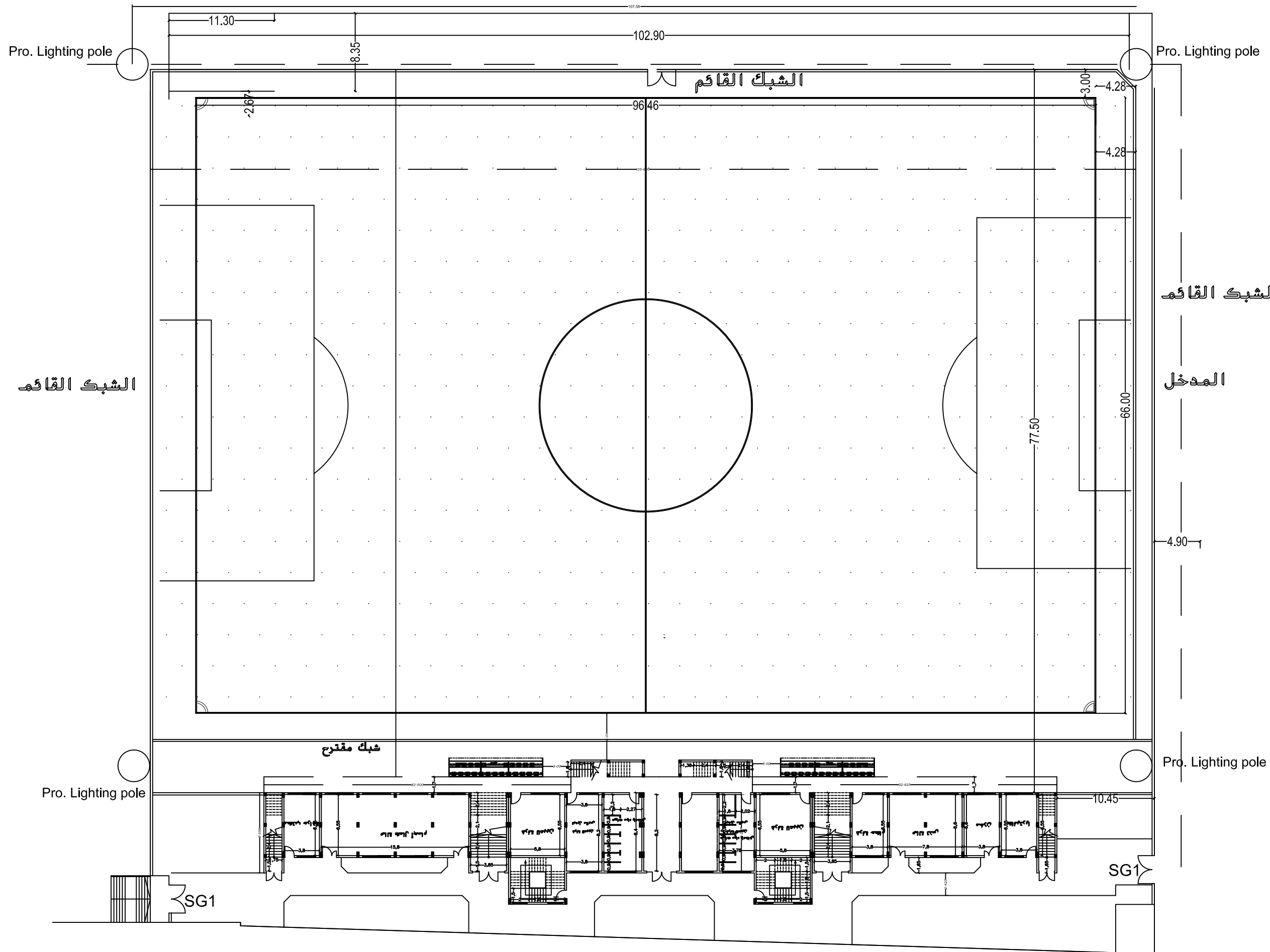
Locations of lighting poles In khanyounis play ground
