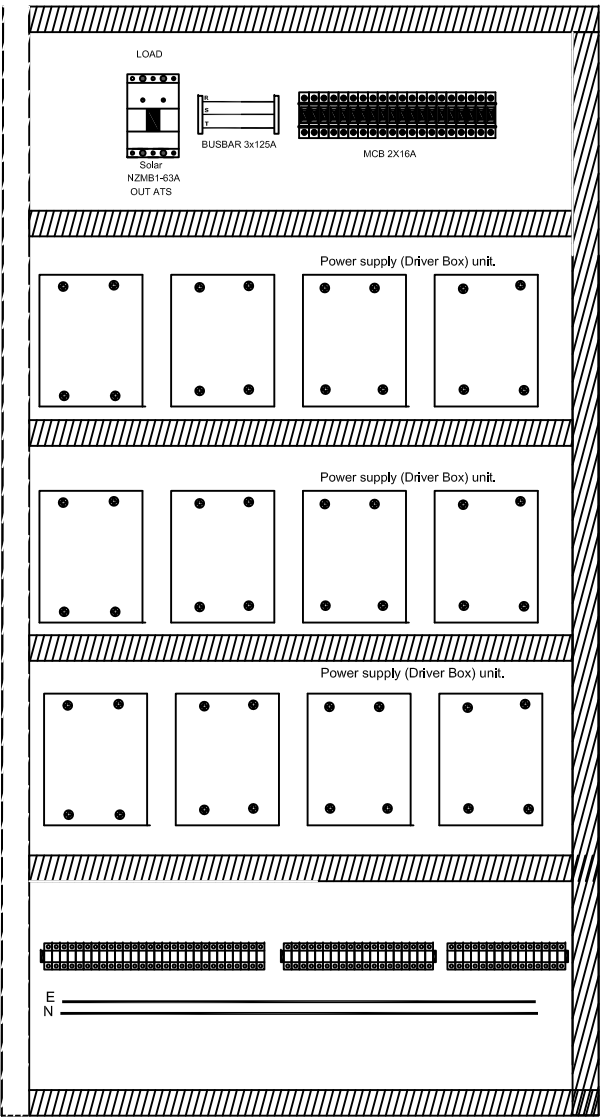
Electrical Pillar
