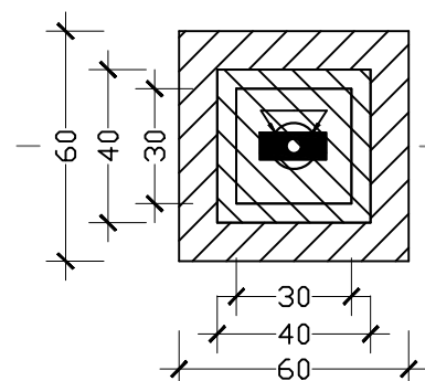
3 E-07 GROUNDING HAND HOLE DETAILS Scale:NOT
