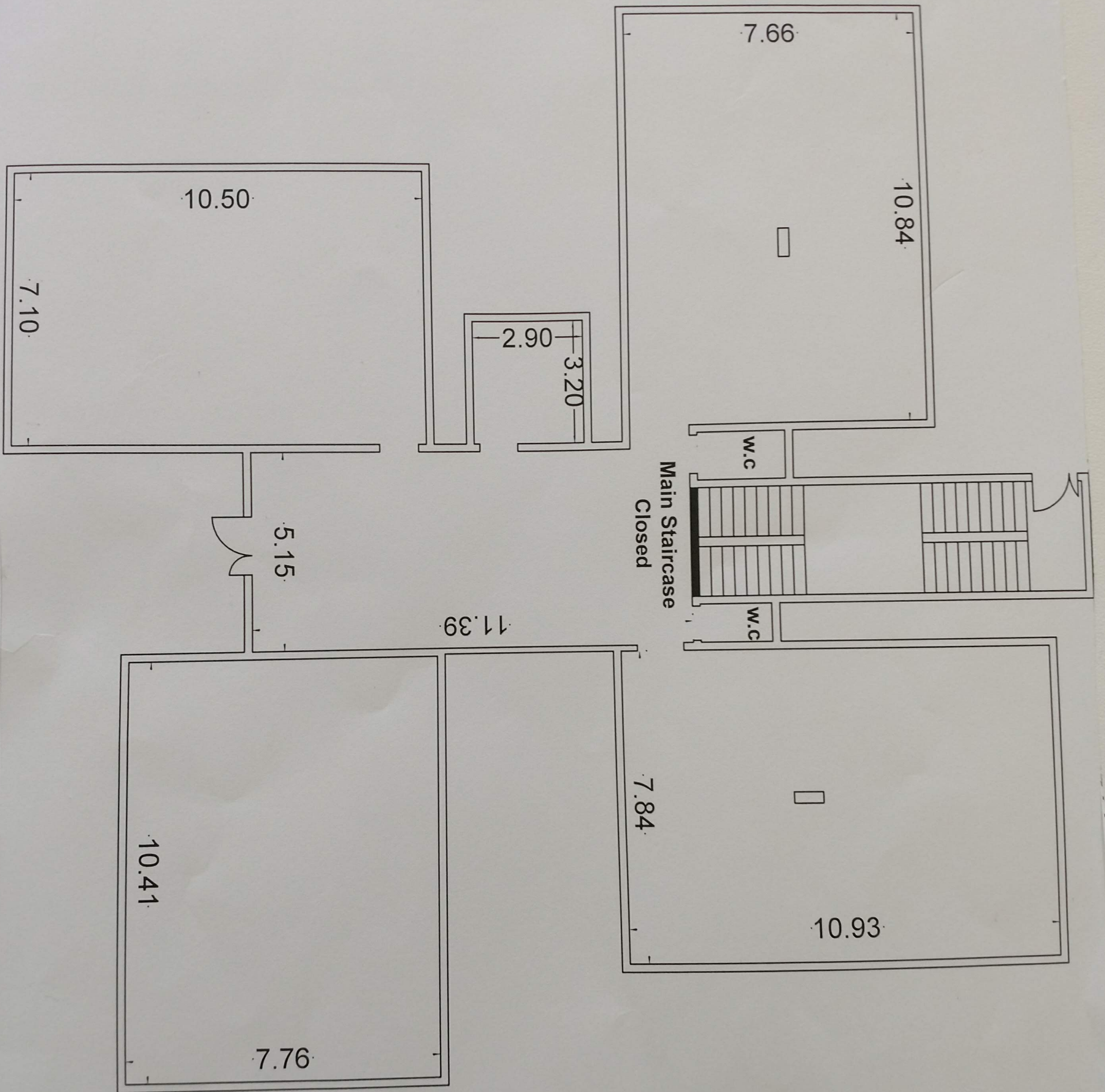
New Interior partition after rehabilitation Ground Floor
