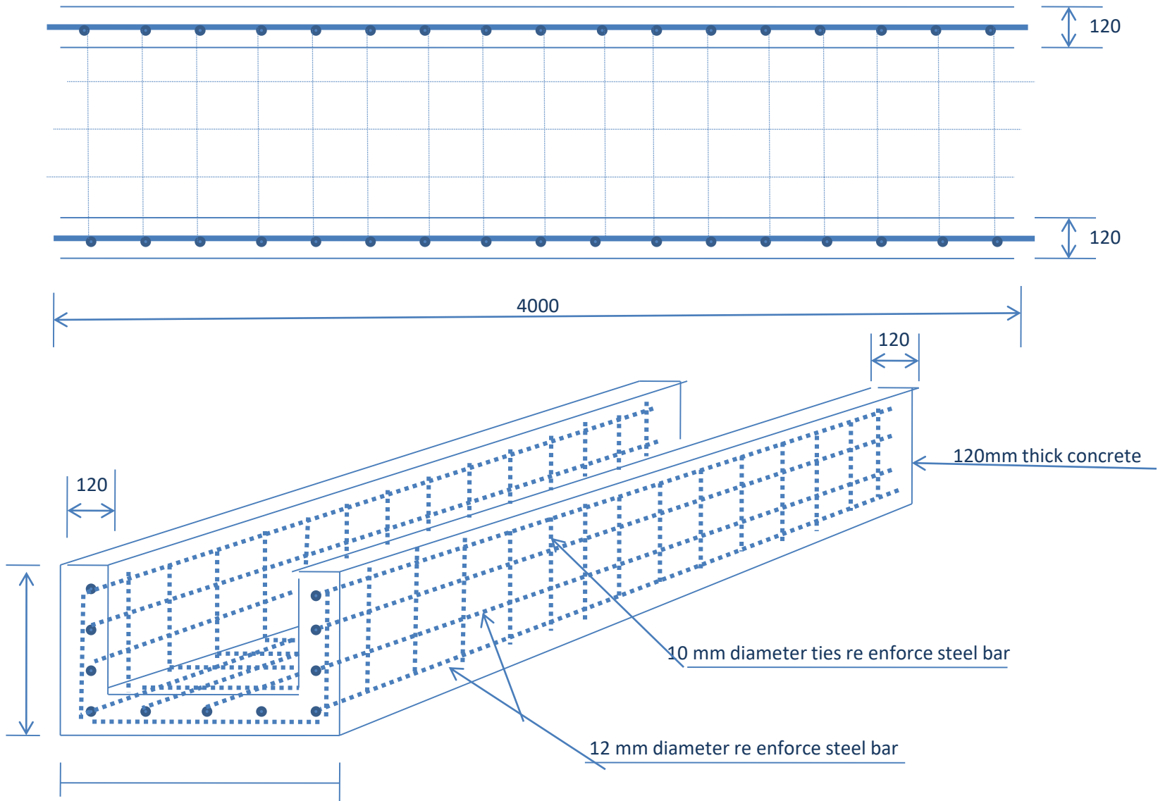
Concrete Drainage Detail
