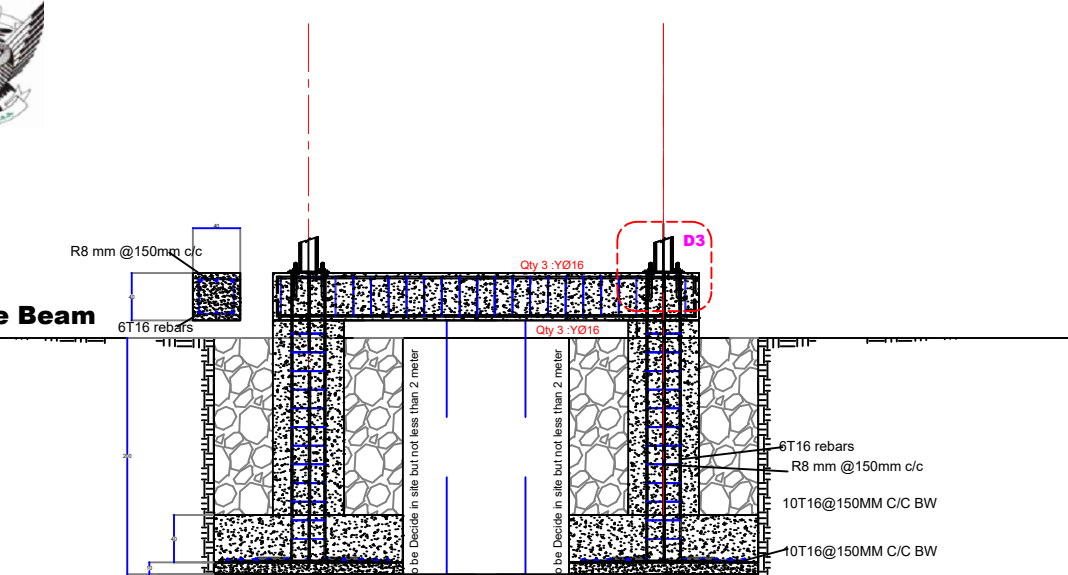
X1-X1 SECTIONAL DETAIL FOUNDATION, SHORT COLUMN & GB. Detail
