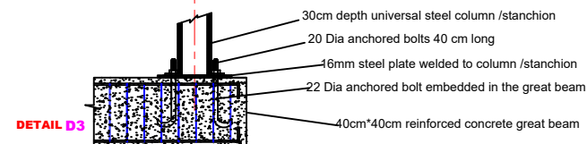
DETAIL D3 FOOT PLATE PLAN
