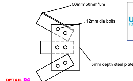
DETAIL D4 Connection plate
