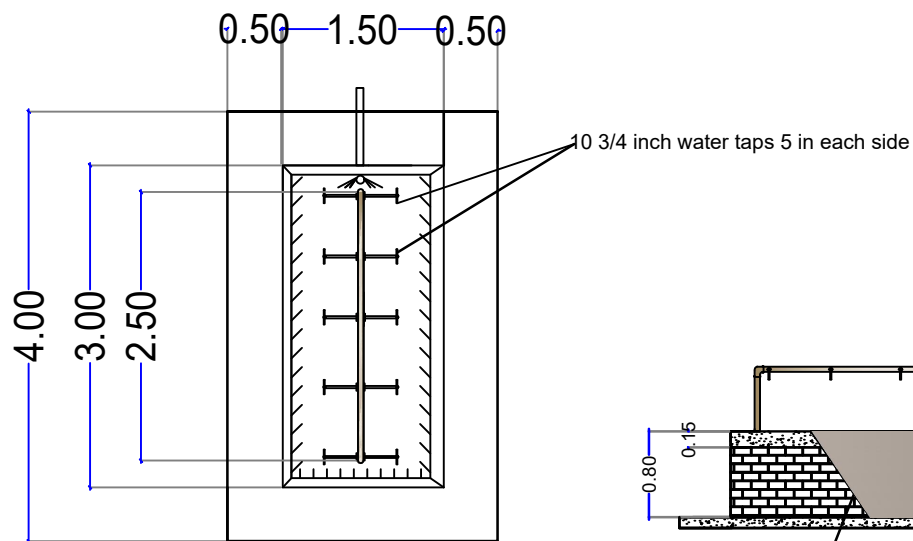
WATER POINT PLAN VIEW
