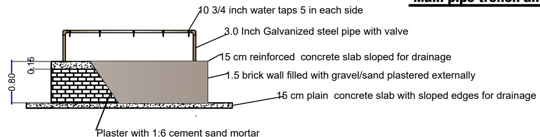
Main pipe trench and pipe
