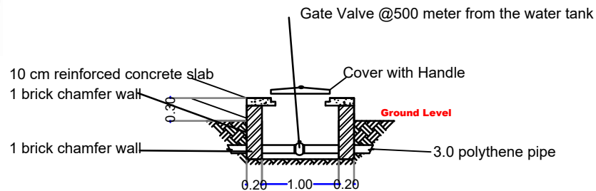
1.2m*1.2m Gate valve chamfer
