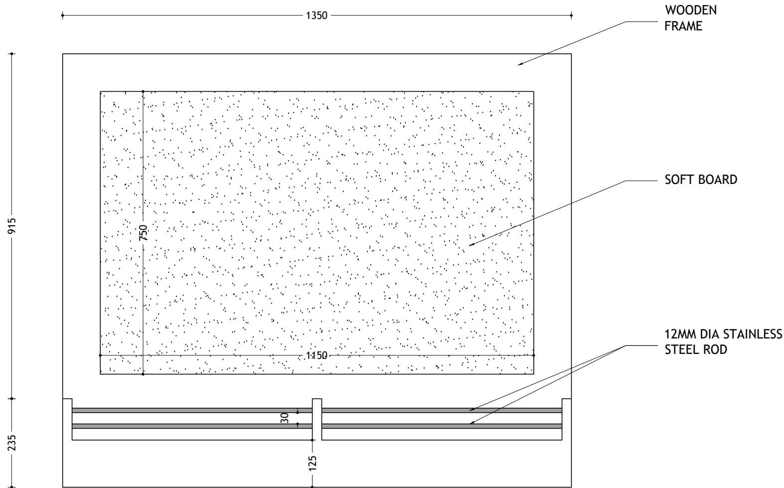
FRONT ELEVATION
