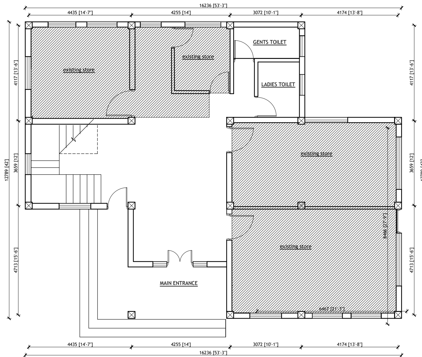
GROUND FLOOR PLAN Total Builtup area = 158 Sq.m Carpet area for EEIC = 64 Sq.m
