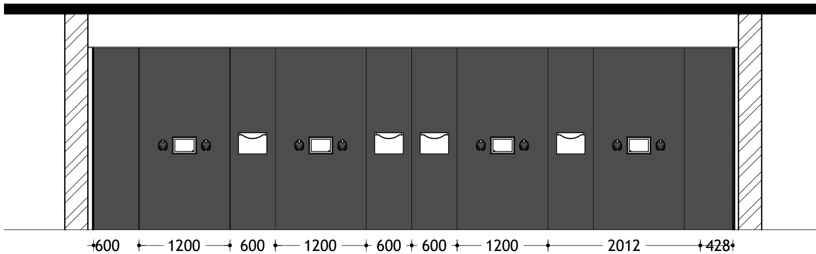
SOUTH WALL ELEVATION
