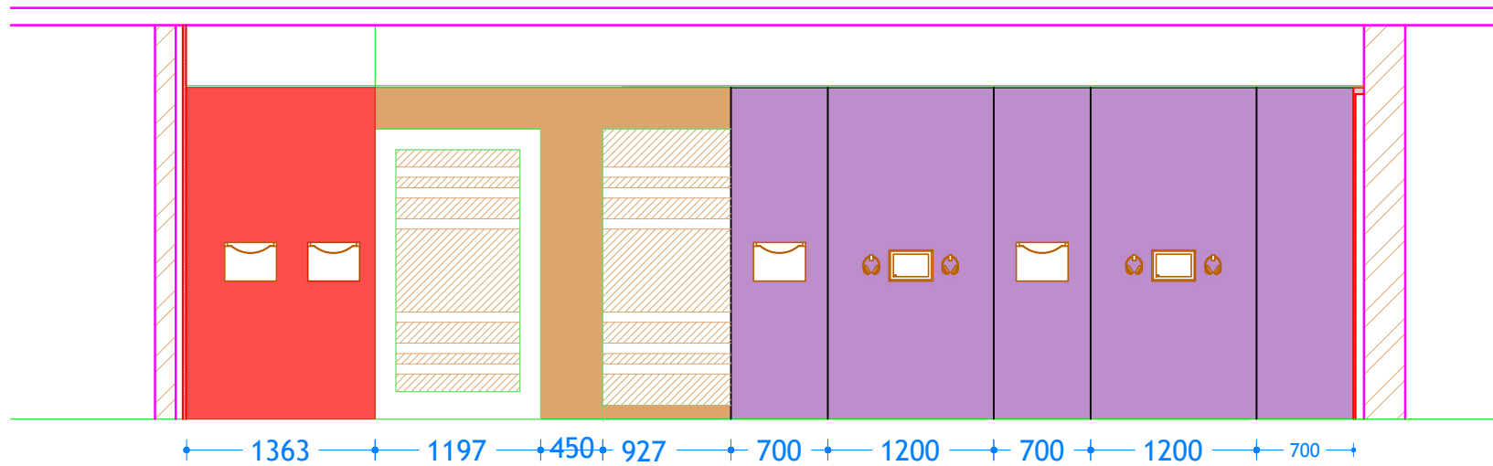
NORTH WALL ELEVATION
