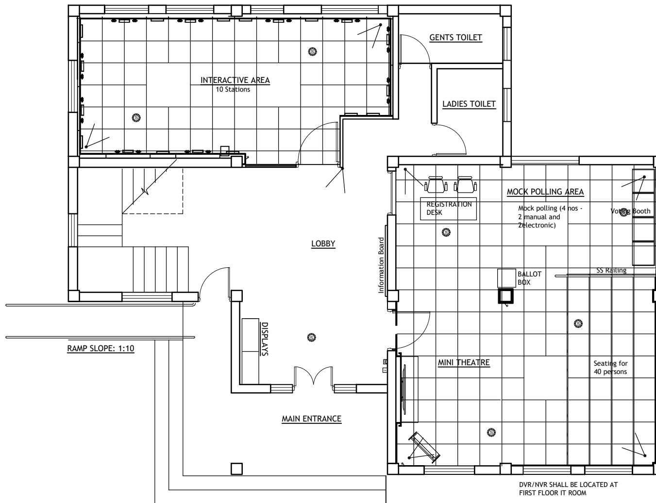
GROUND FLOOR PLAN Total Builtup area = 158 Sq.m Carpet area for EEIC = 64 Sq.m
