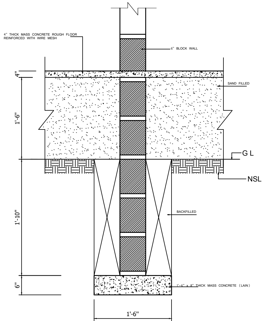
SECTION S-S PROPOSED
