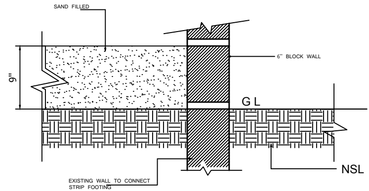
SECTION F-F EXISTING
