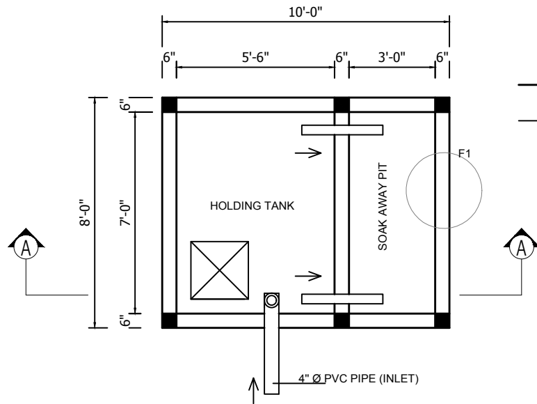
SEPTIC TANK PLAN
