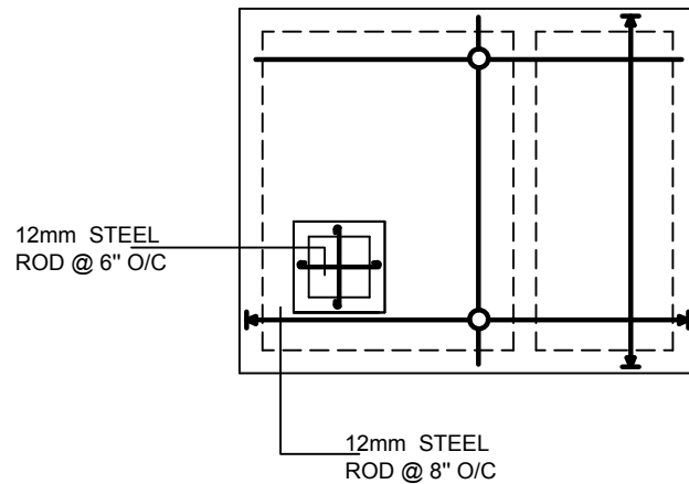
SLAB PLAN
