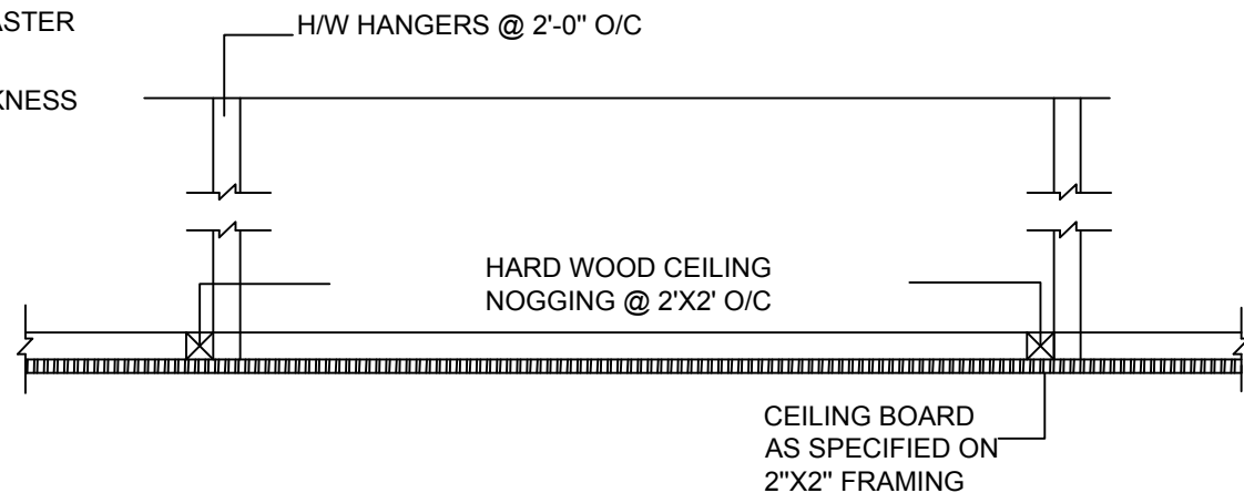
SECTION @ B
