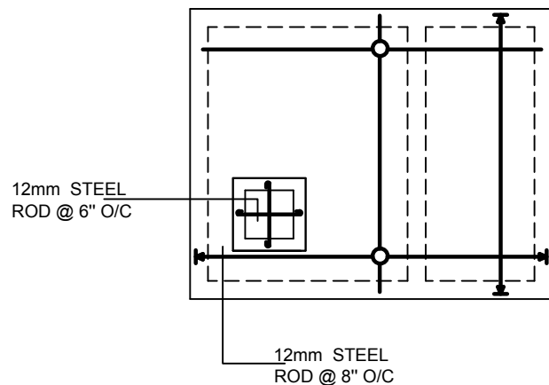
SLAB PLAN
