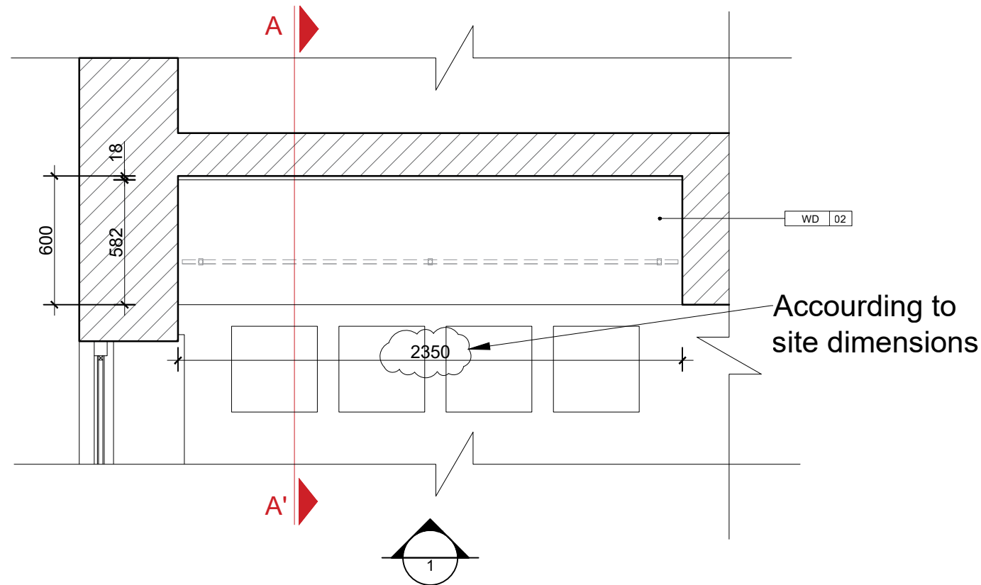
1 Bar Table Plan UN YEREVAN OFFICE ROOM N405 SCALE 1:25
