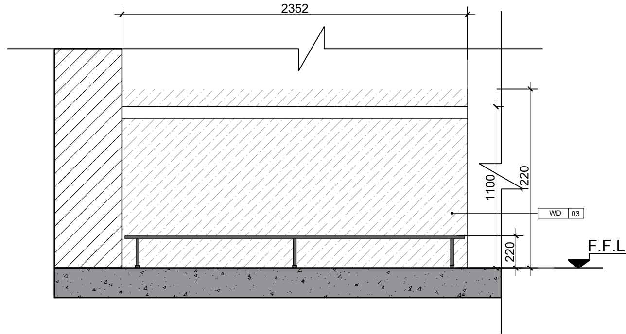
2 Elevation 1 UN YEREVAN OFFICE ROOM N405 SCALE 1:25
