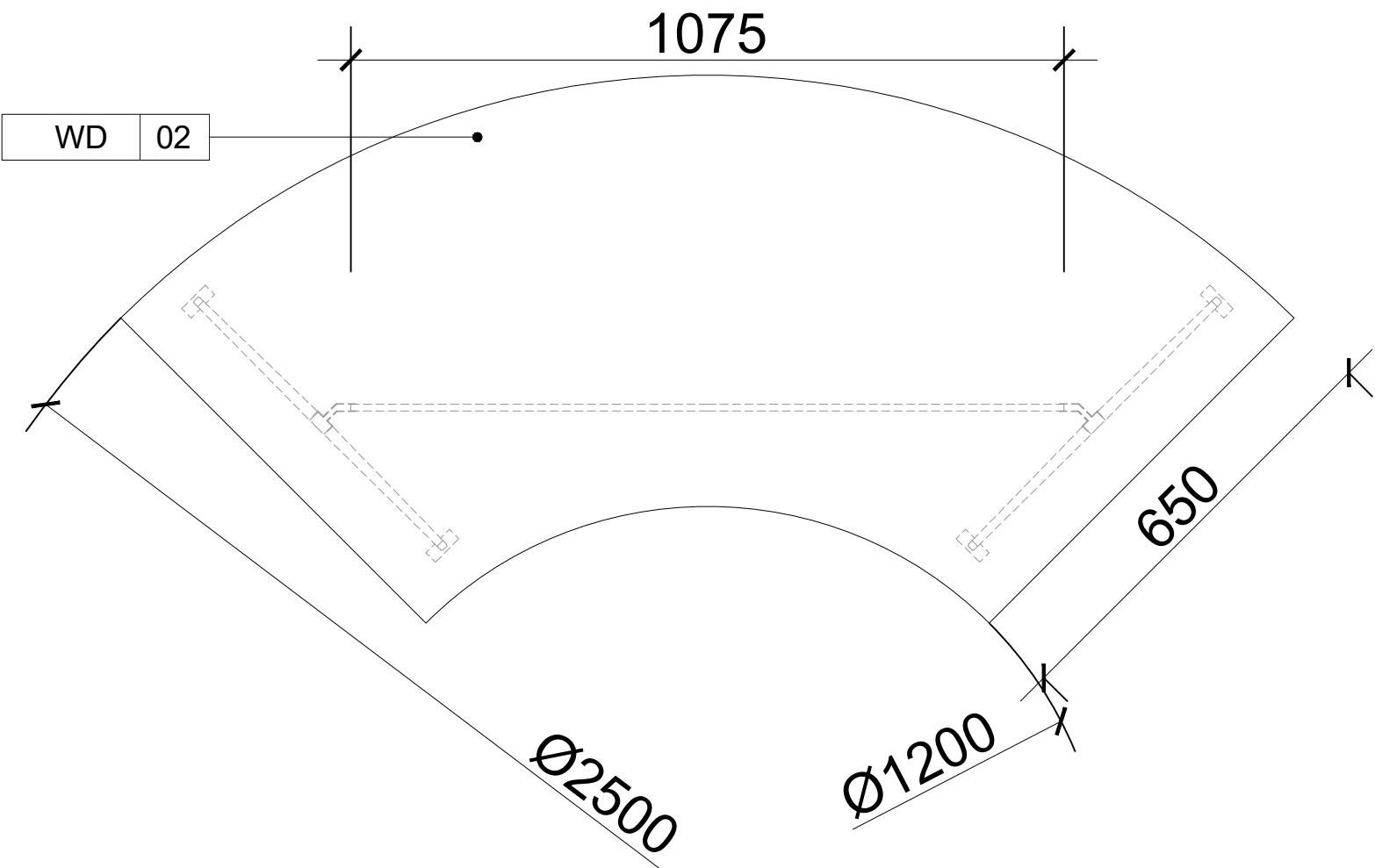
1 Table Plan UN YEREVAN OFFICE ROOM N405 SCALE 1:20
