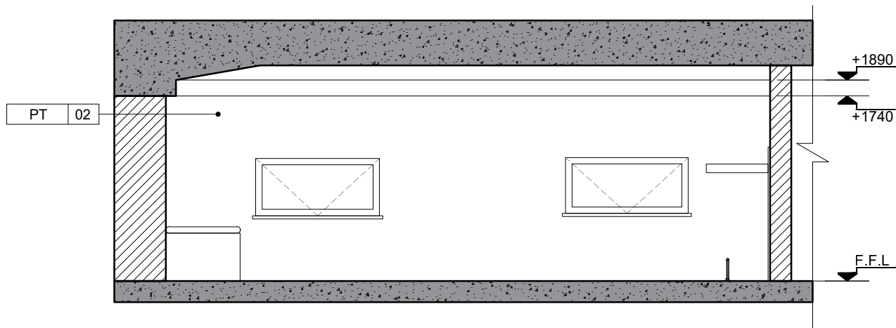
2 Elevation 4 UN YEREVAN OFFICE ROOM N405 SCALE 1:50
