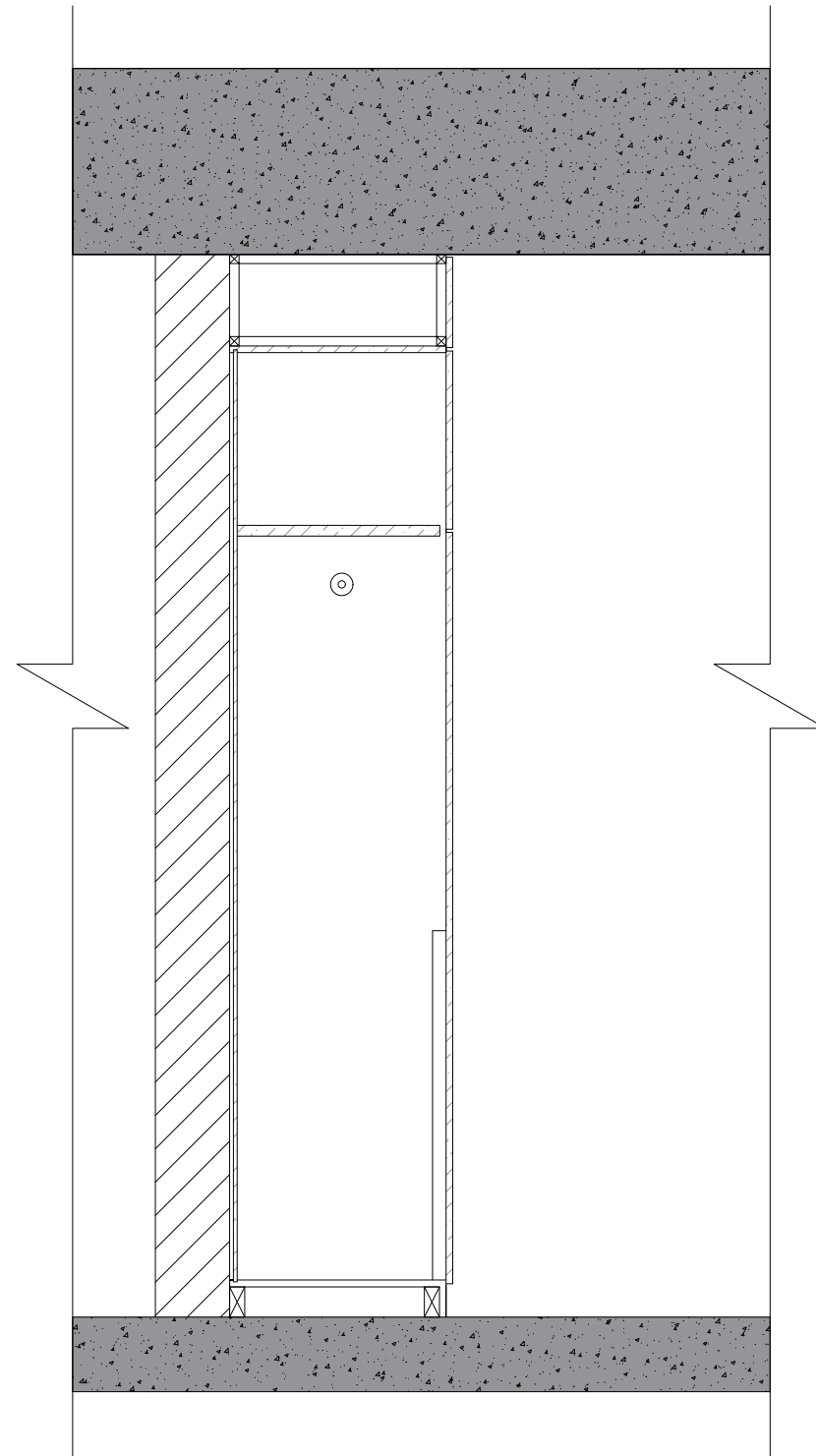
3 Section AA' UN YEREVAN OFFICE ROOM N405 SCALE 1:20
