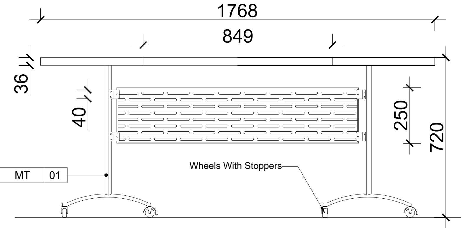
2 Elevation 1 UN YEREVAN OFFICE ROOM N405 SCALE 1:20
