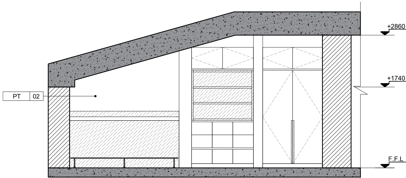
2 Elevation 1 UN YEREVAN OFFICE ROOM N405 SCALE 1:50
