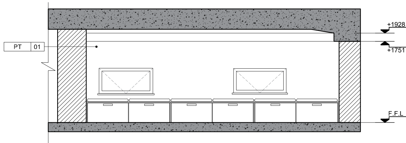
2 Elevation 3 UN YEREVAN OFFICE ROOM N405 SCALE 1:50
