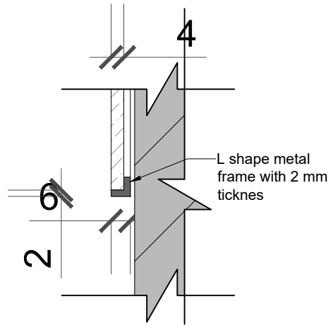
4 Room 314 Detail 3 UNDP Yerevan Offices SCALE 1:5
