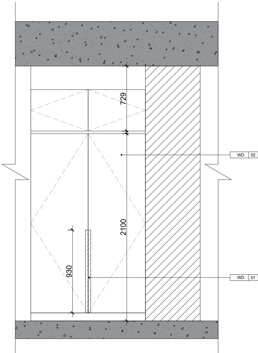
2 Elevation 1 UN YEREVAN OFFICE ROOM N405 SCALE 1:25
