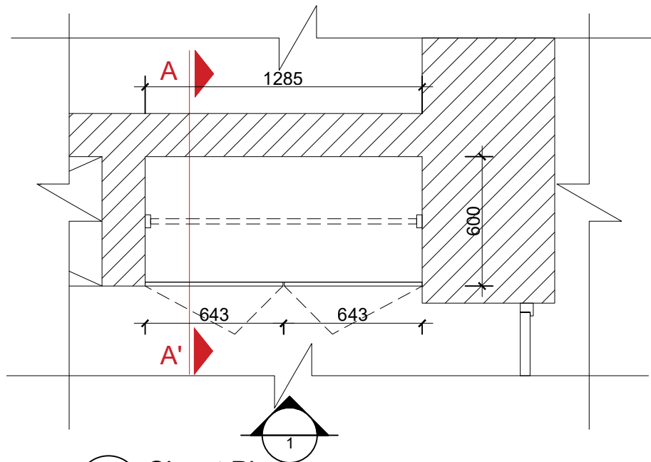
1 Closet Plan UN YEREVAN OFFICE ROOM N405 SCALE 1:25
