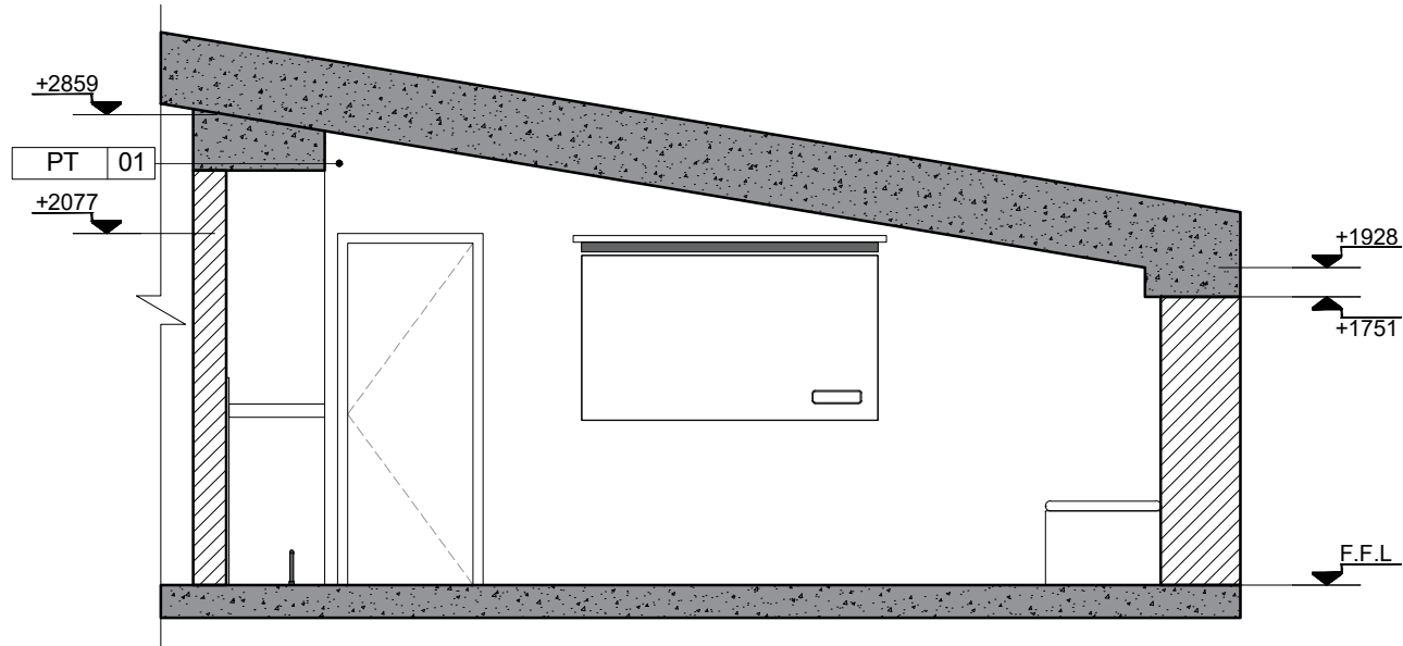
2 Elevation 2 UN YEREVAN OFFICE ROOM N405 SCALE 1:50
