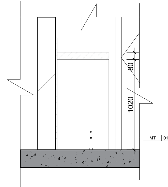
3 Section AA' UN YEREVAN OFFICE ROOM N405 SCALE 1:25
