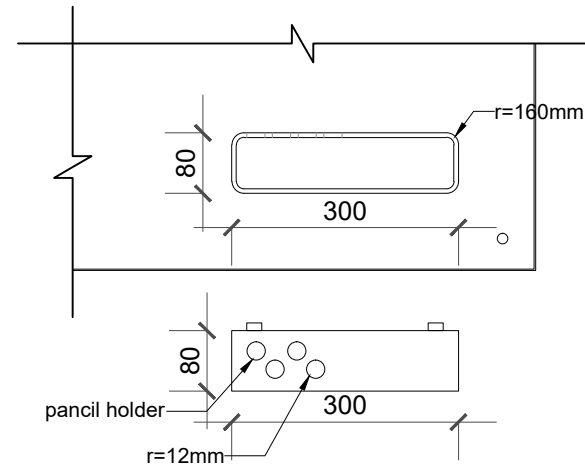
1 Room 314 Detail 2 UNDP Yerevan Offices SCALE 1:10
