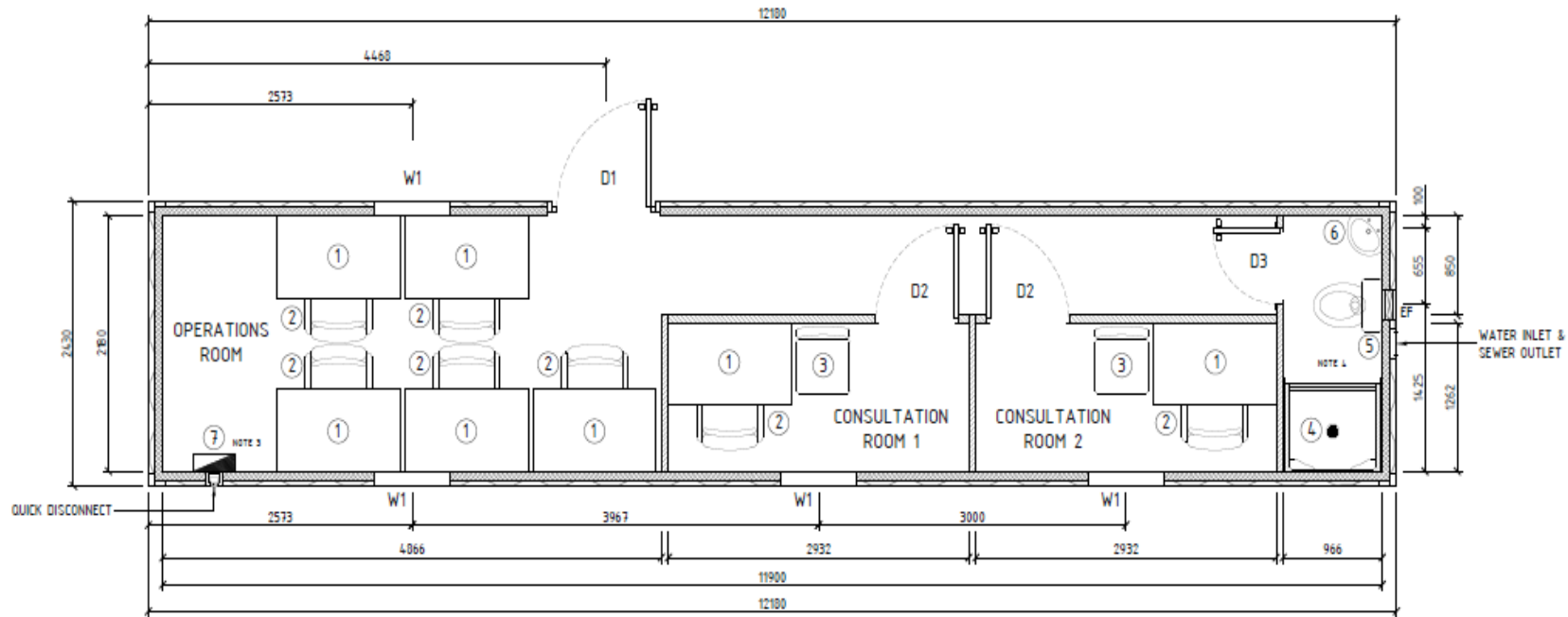
FLOOR PLAN SCALE 1/25
