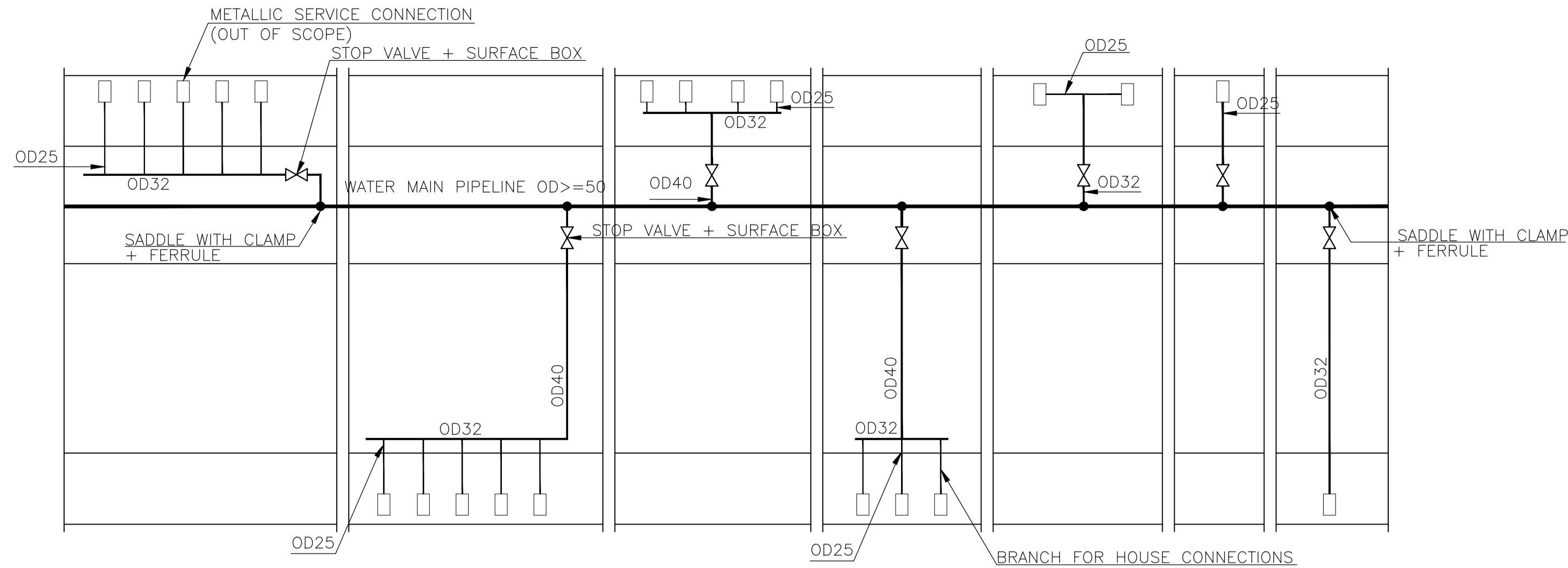
HOUSE CONNECTION TYPES – SCHEMATIC LAYOUT N.T.S.
