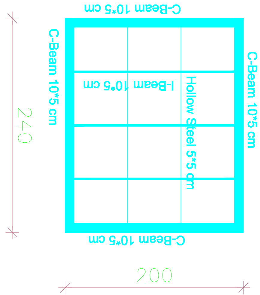
Floor Steel Plan
