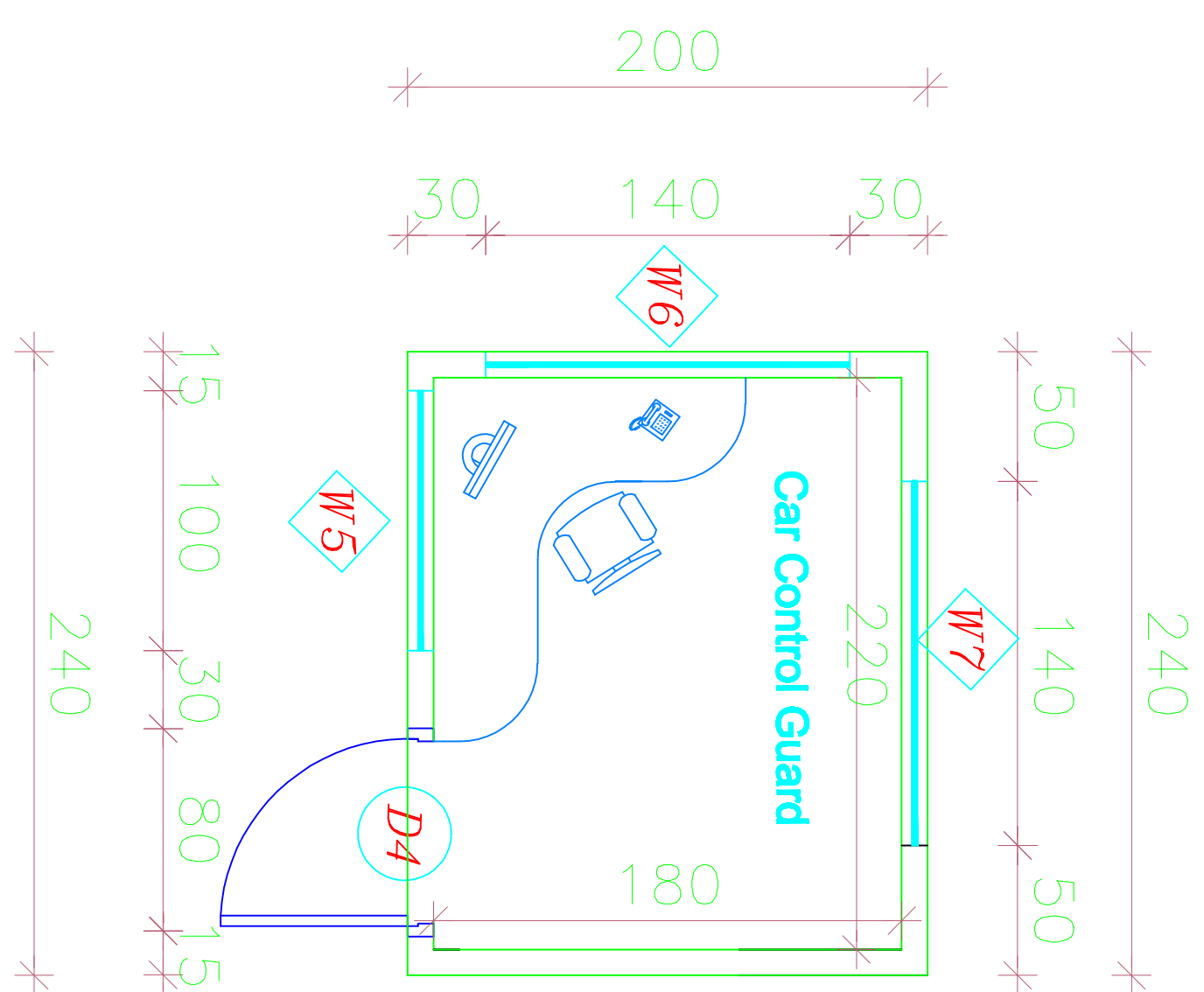
Car Control Guard Booth Plan
