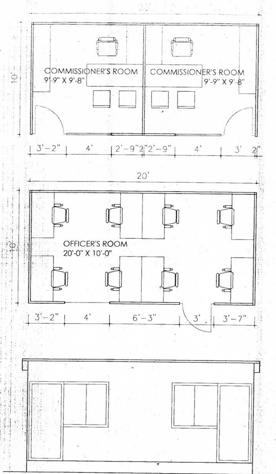
FRONT ELEVATION
