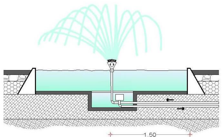
Figure 5 example of the fountain but with higher borders and overflow
