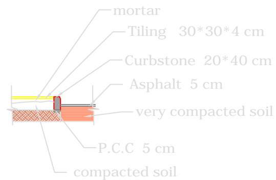
TYPICAL DETAIL OF TILING AREA scale 1/100
