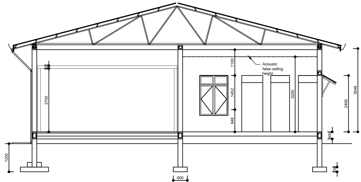
CROSS SECTION (1:100)
