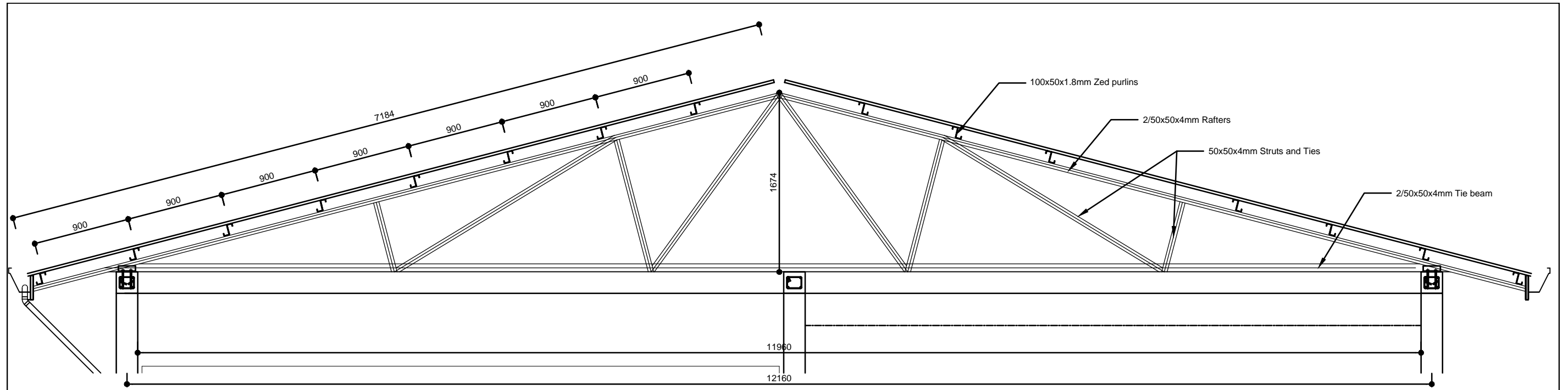
TRUSS DETAILS (1:50)
