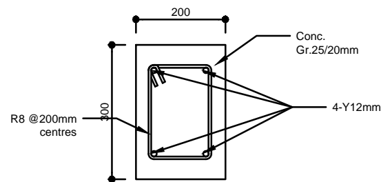
SECTION THRU GBM
