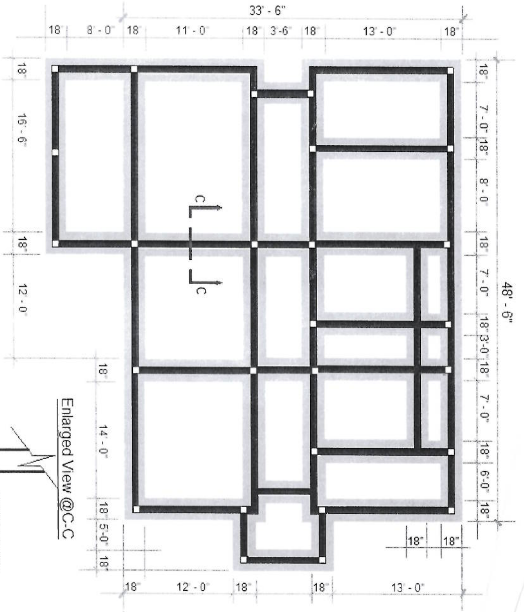
Foundation Plan
