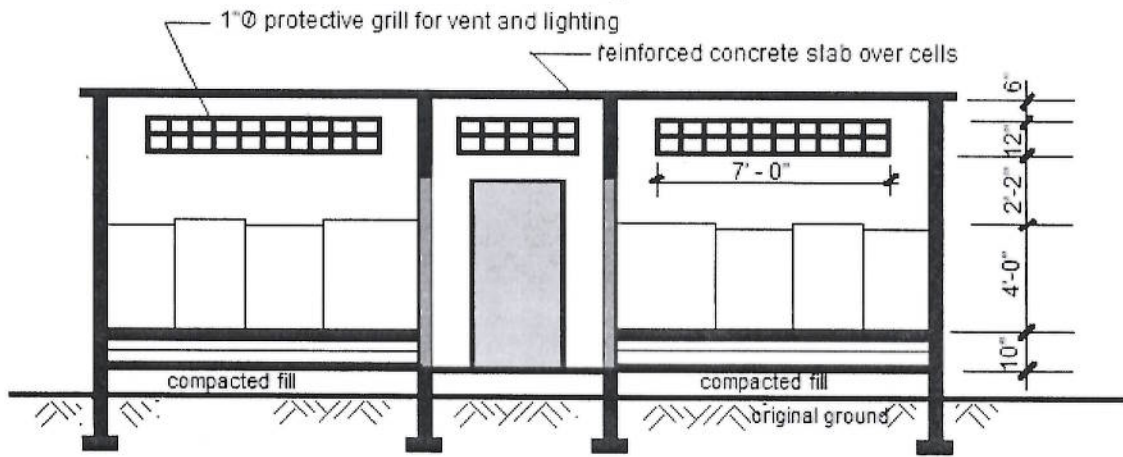
Detailed @A-A
