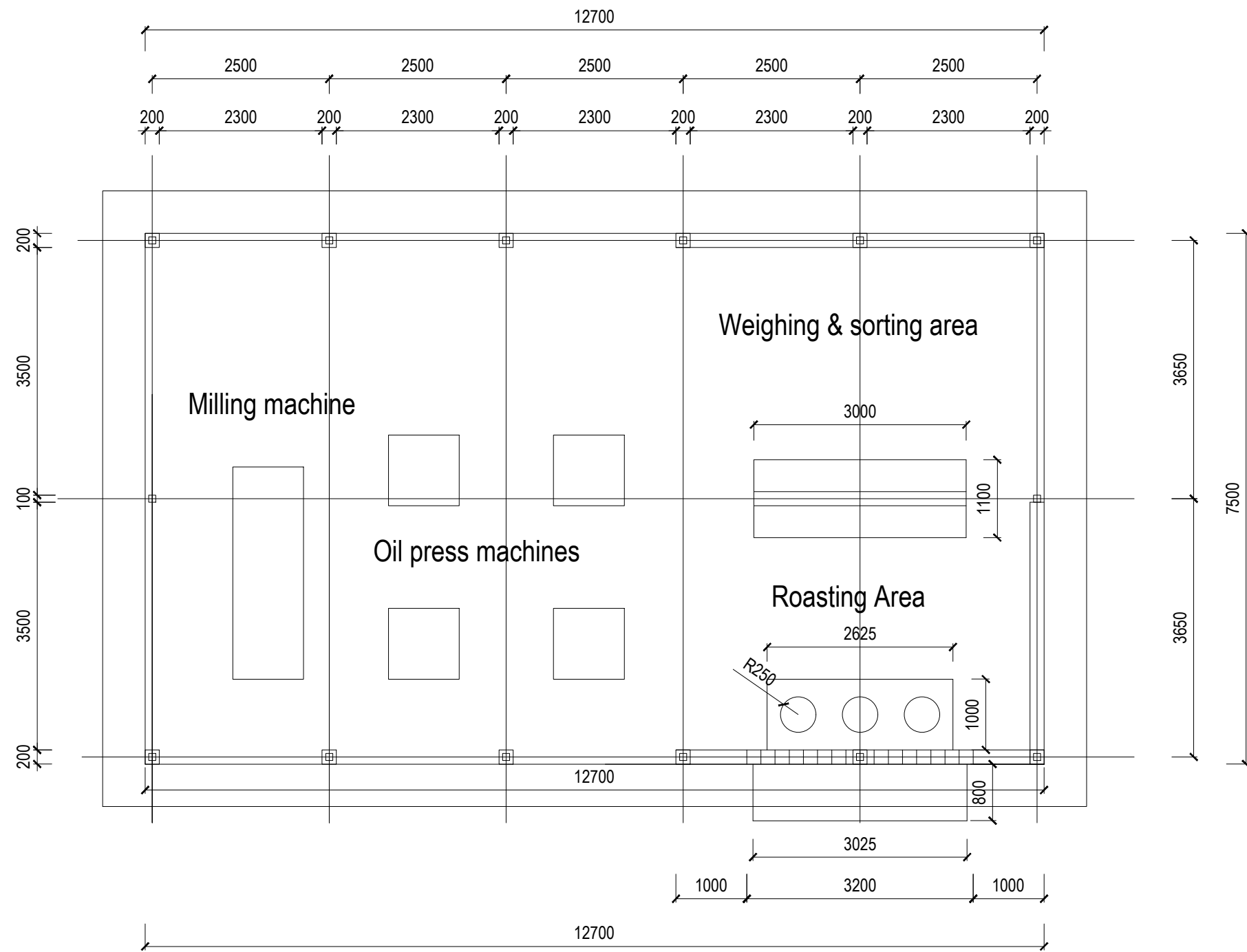
GROUND LAYOUT PLAN
