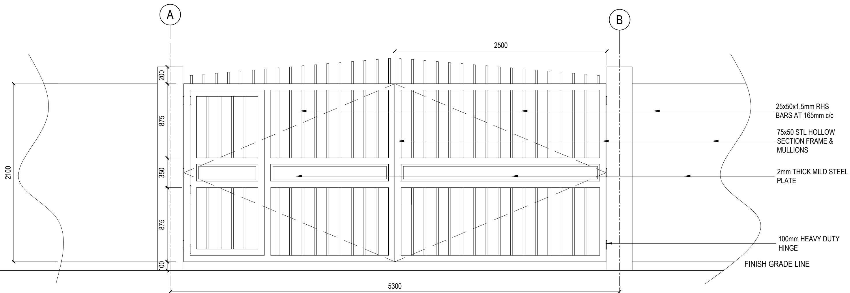
TYPICAL GATE ELEVATION
