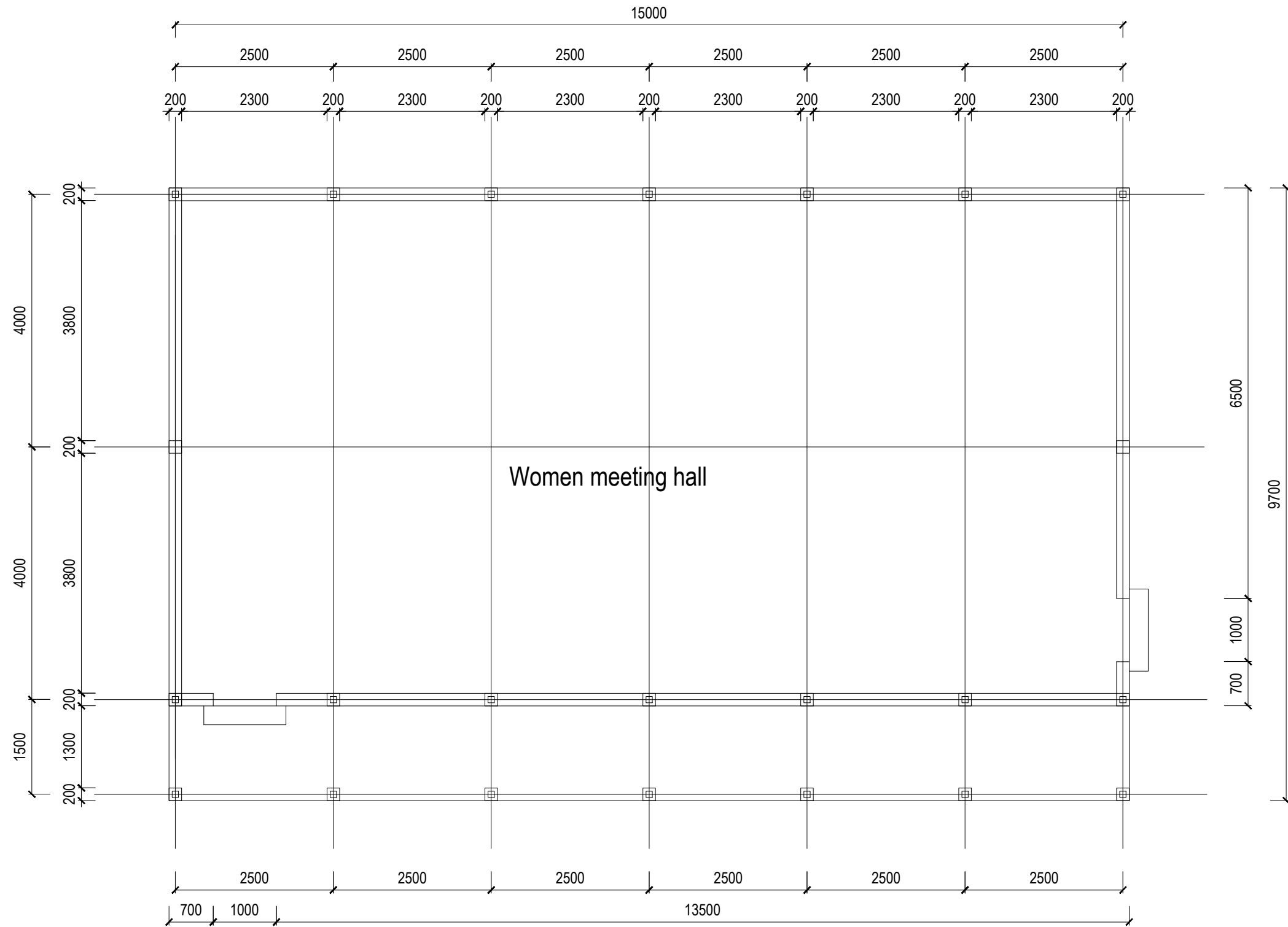
LAYOUT PLAN
