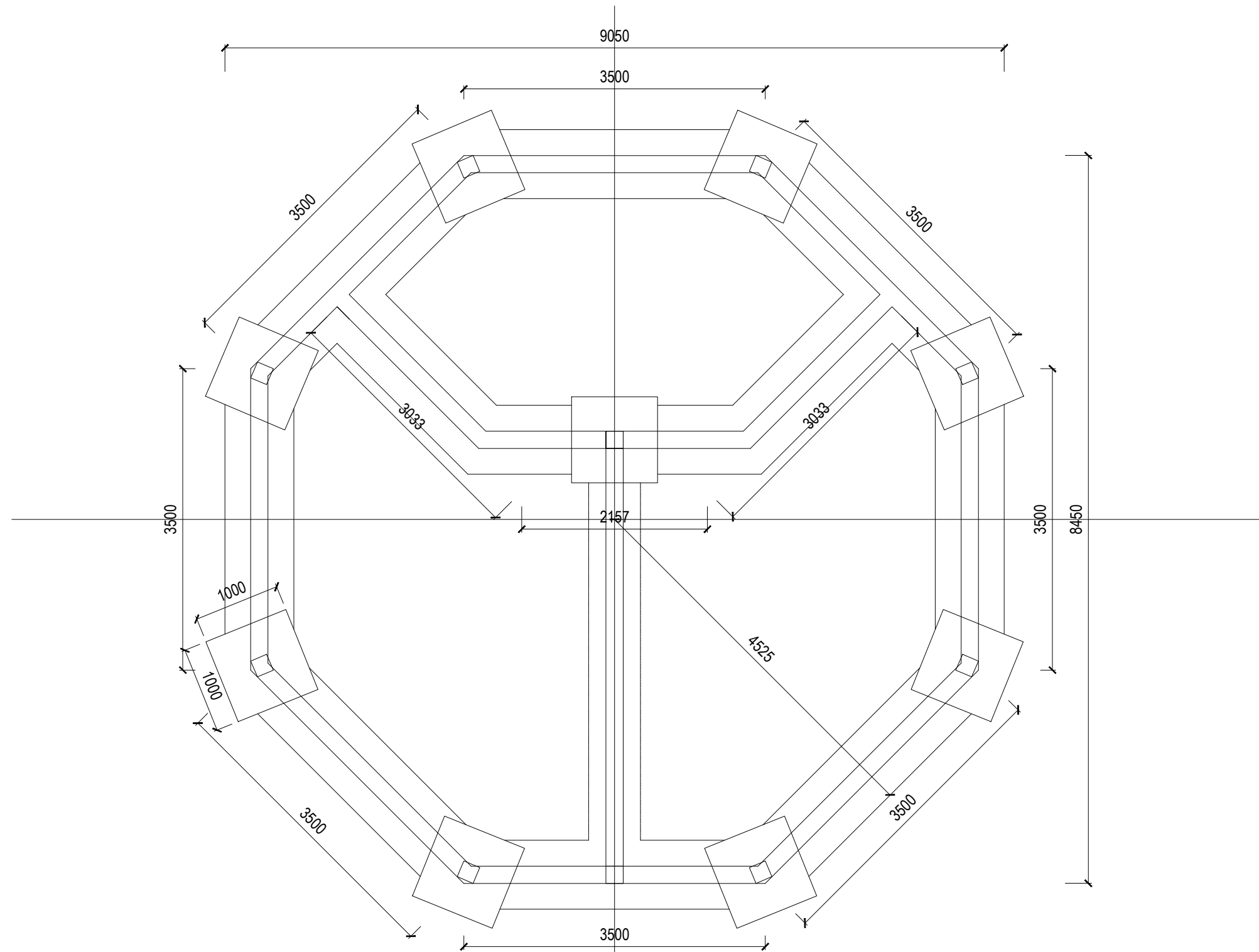
FOUNDATION PLAN
