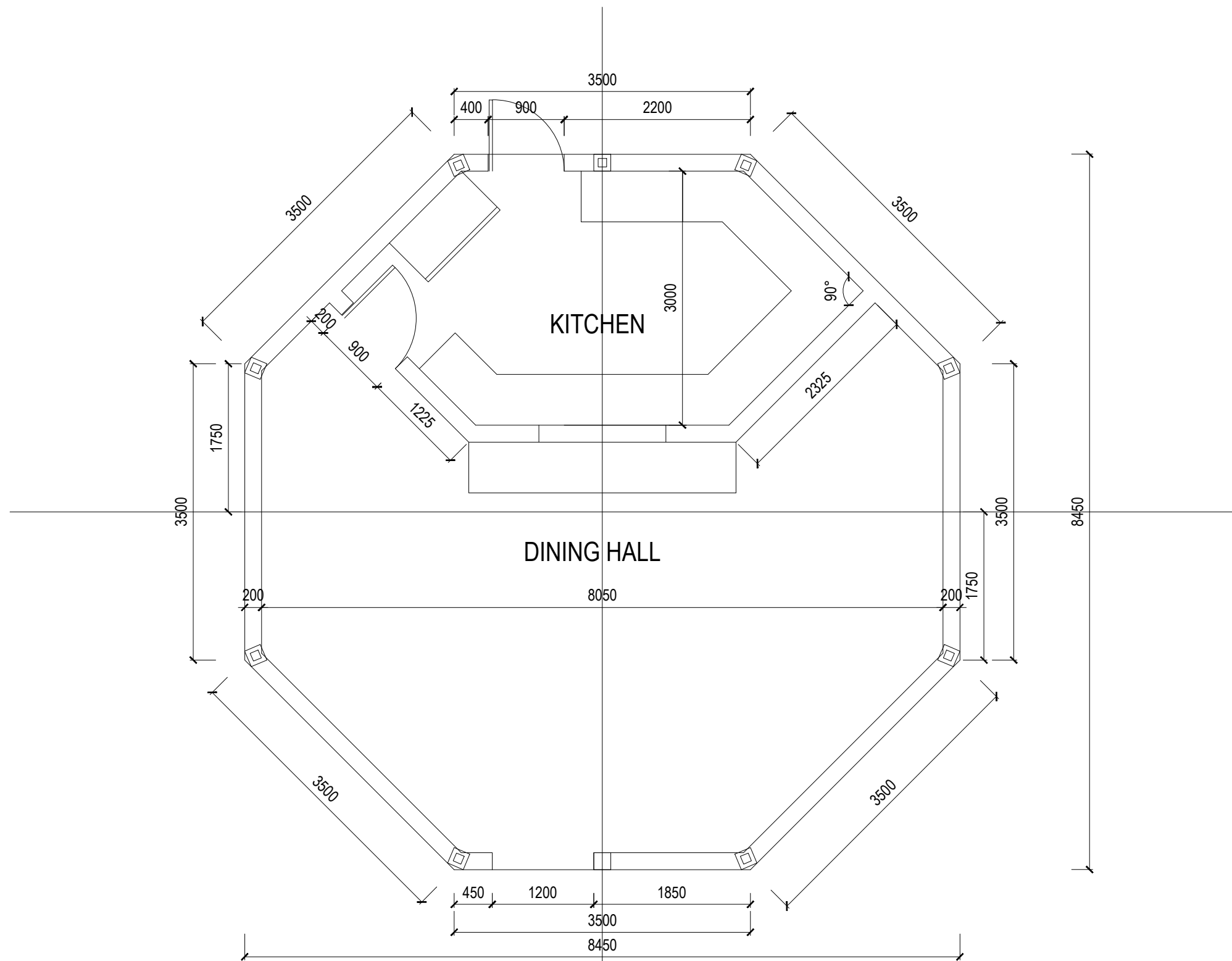
LAYOUT PLAN
