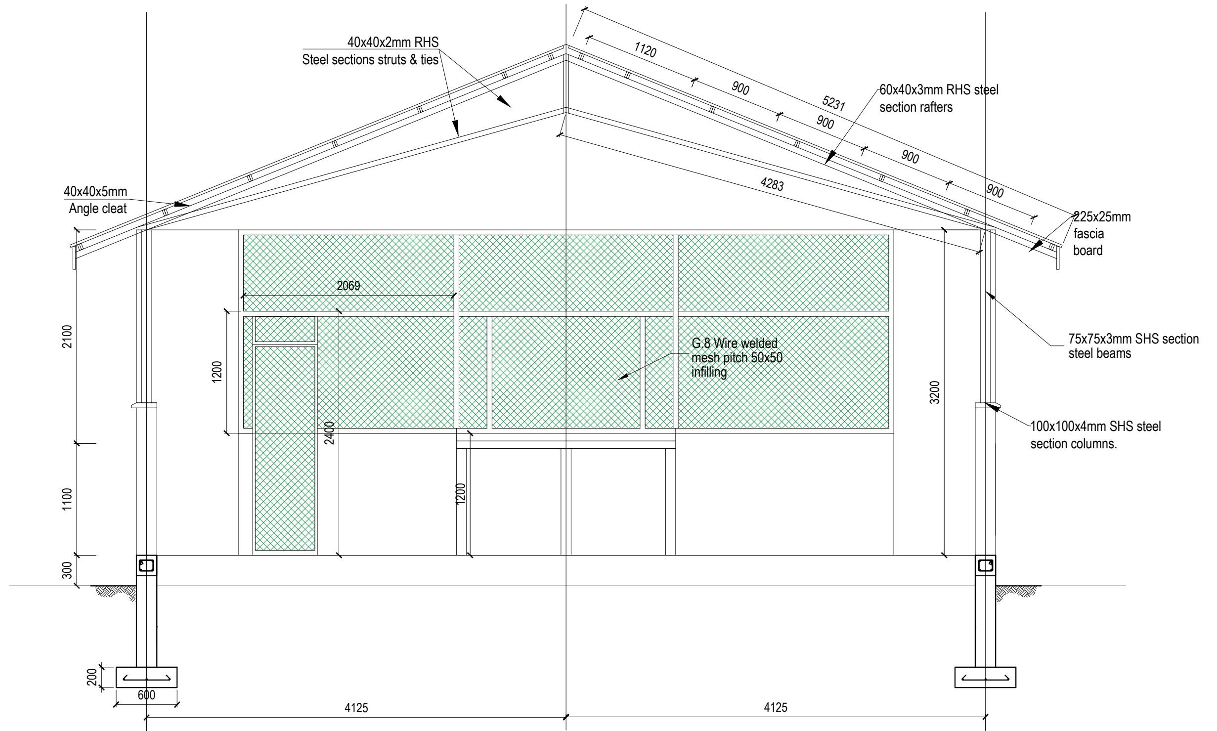
SECTIONAL ELEVATION
