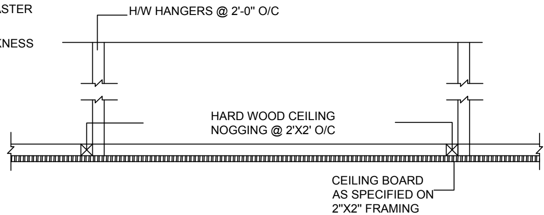
SECTION @ B
