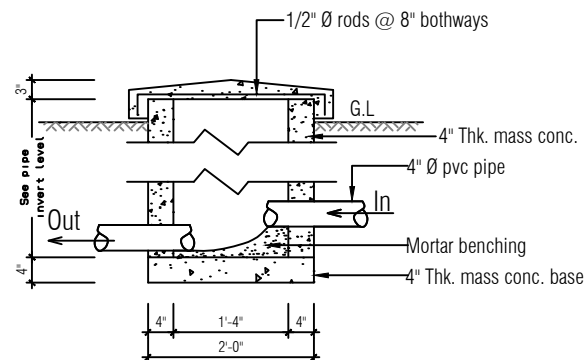
SECTION M1-M1
