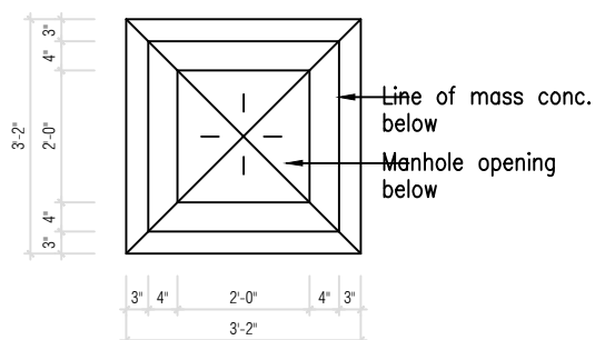
PLAN OF MANHOLE COVER
