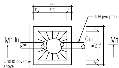
MANHOLE PLAN
