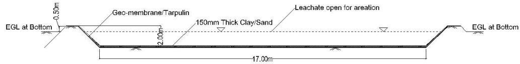
Section of Leachate Pond
