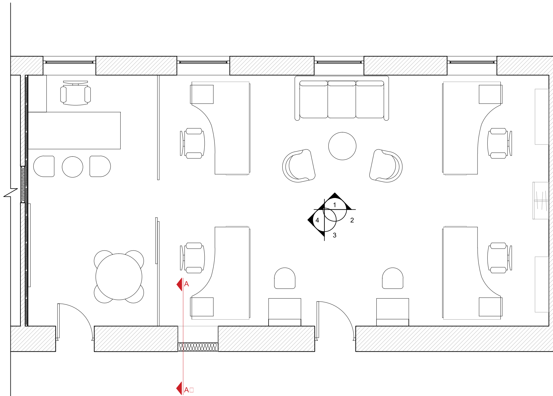
1 Furniture Layout Plan UN RC OFFICE YEREVAN SCALE 1:50
