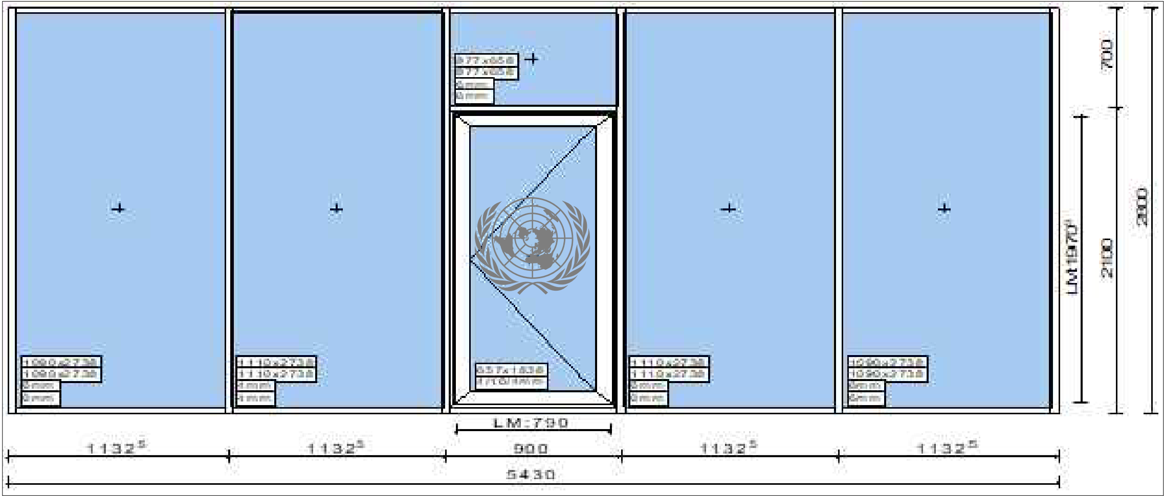
2 Seperating Wall Elevation Option 2 UN RC OFFICE YEREVAN SCALE 1:50
