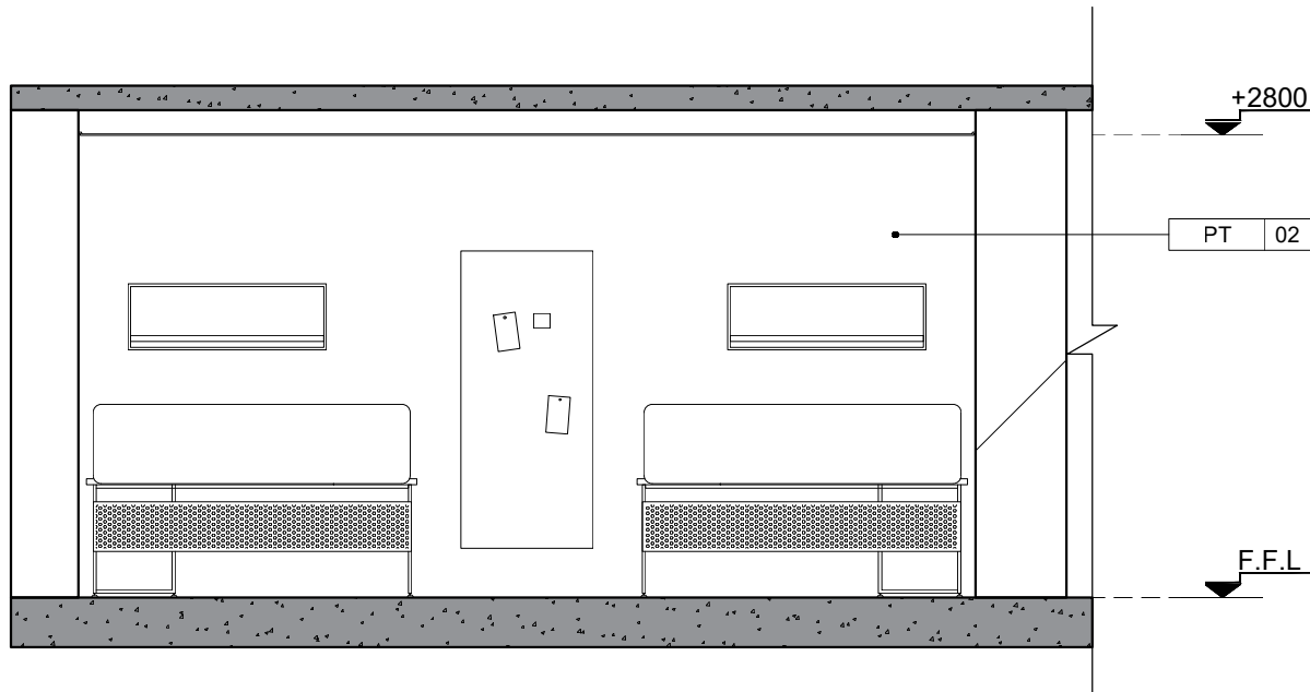
2 Elevation2 UN RC OFFICE YEREVAN SCALE 1:50
