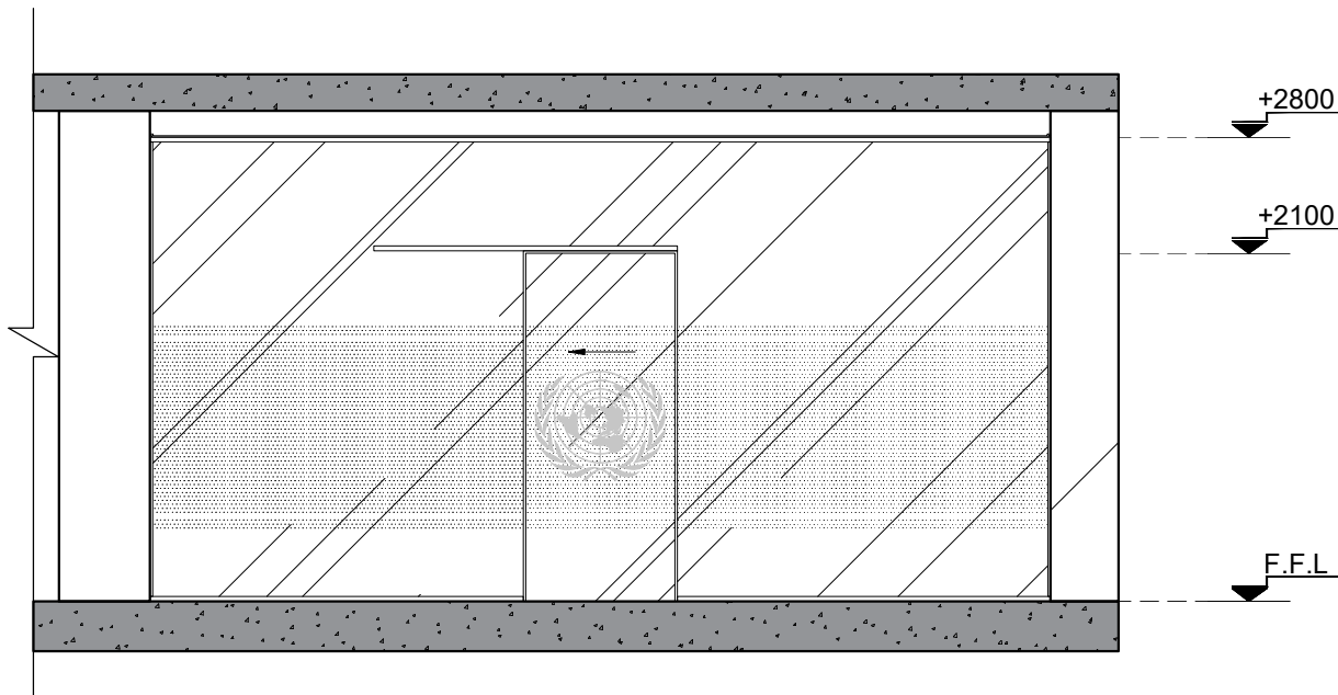
2 ELEVATION 4 UN RC OFFICE YEREVAN SCALE 1:50
