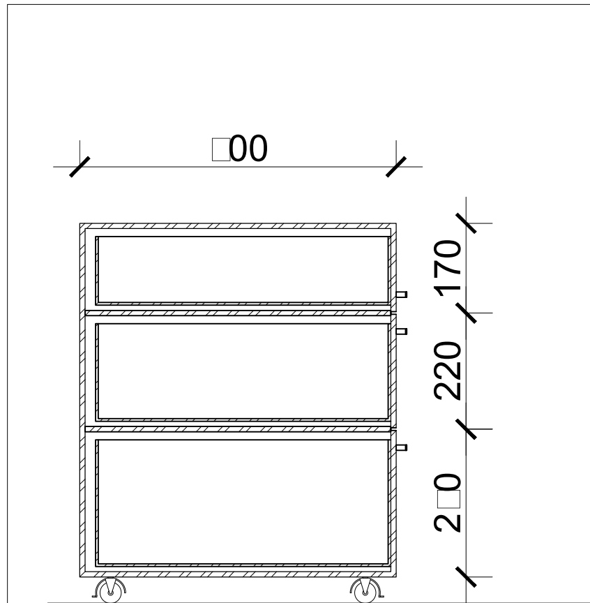
3 S AA UN RC OFFICE YEREVAN SCALE 1:10
