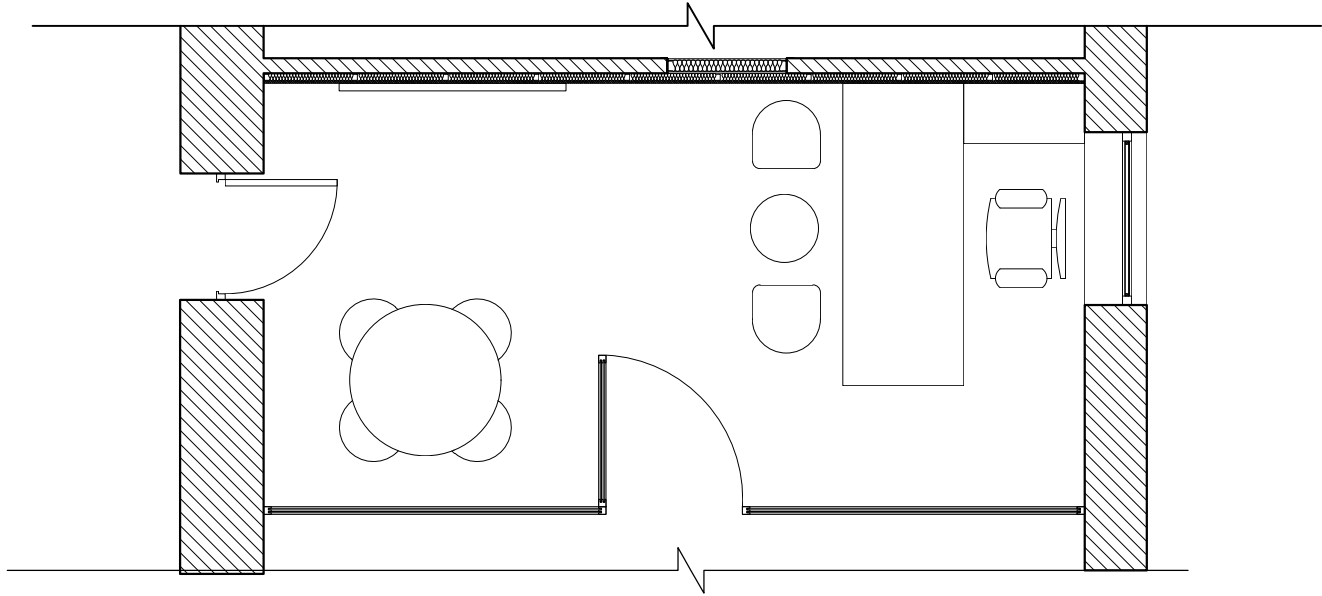
1 Seperating Wall Plan Option 2 UN RC OFFICE YEREVAN SCALE 1:50
