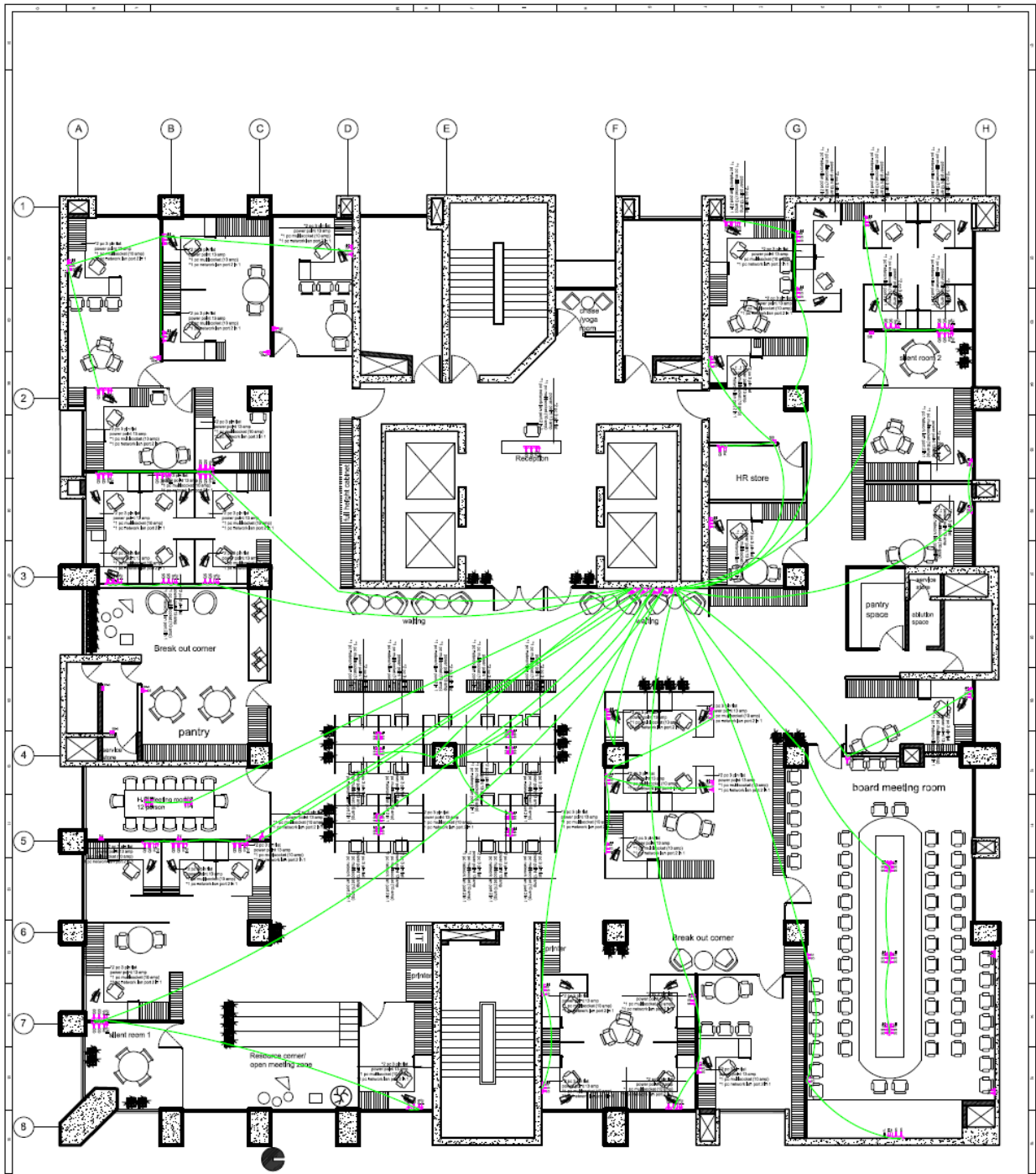
ELECTRICAL FIXTURE & CONDUIT LAYOUT FOR 19th FLOOR
