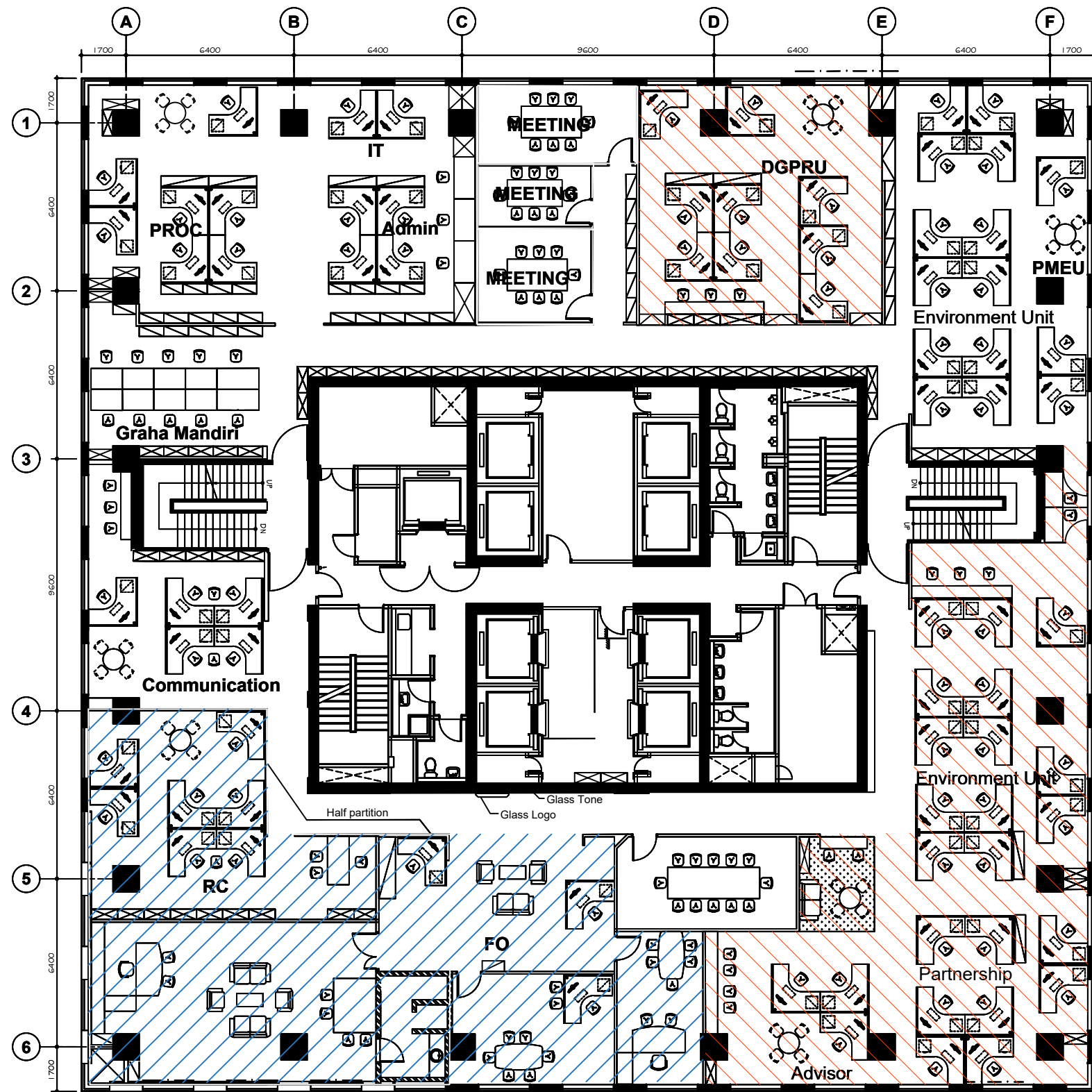
1 FLOOR PLAN FLOOR 9 - EXISTING INT 1968 UNDP OFFICE SCALE 1 : 200
