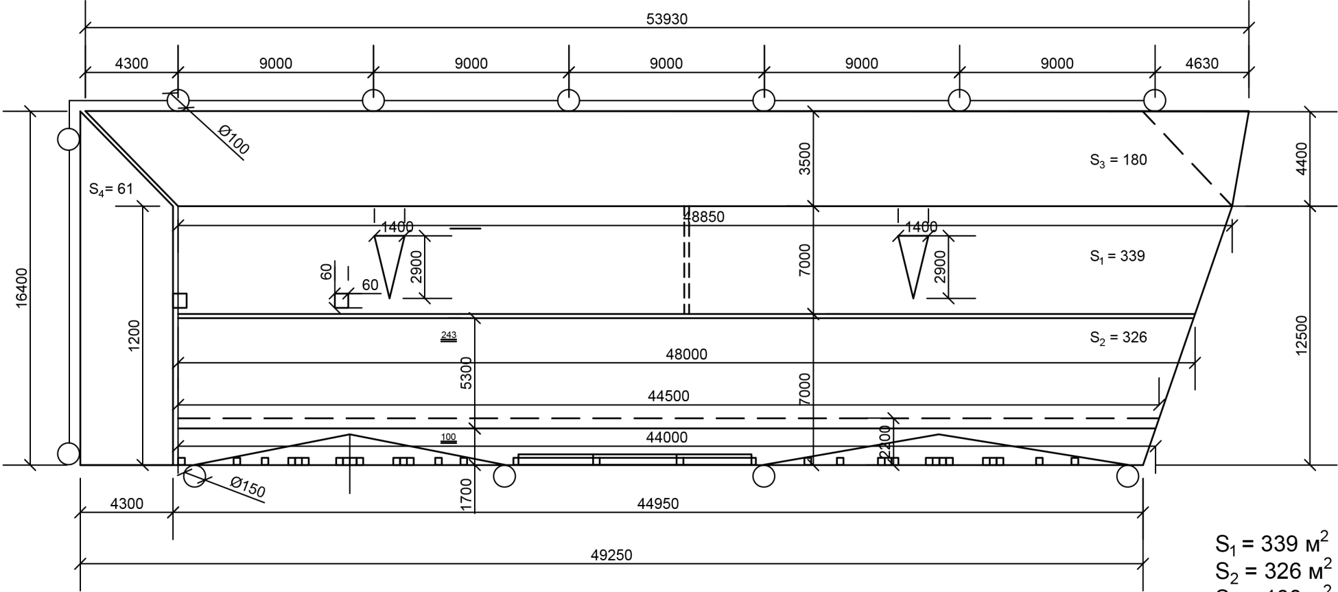
Drawing: Roof of Sukhumi State College
