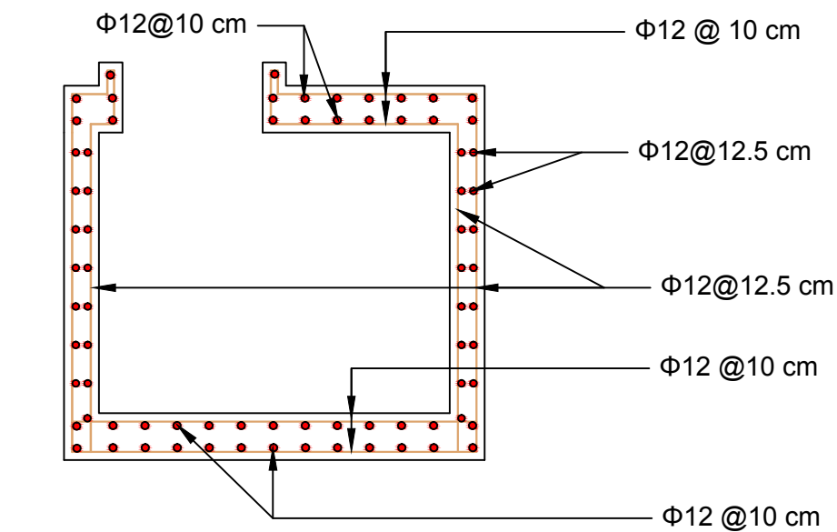
Manhole Chamber Reinforced Concrete Details
