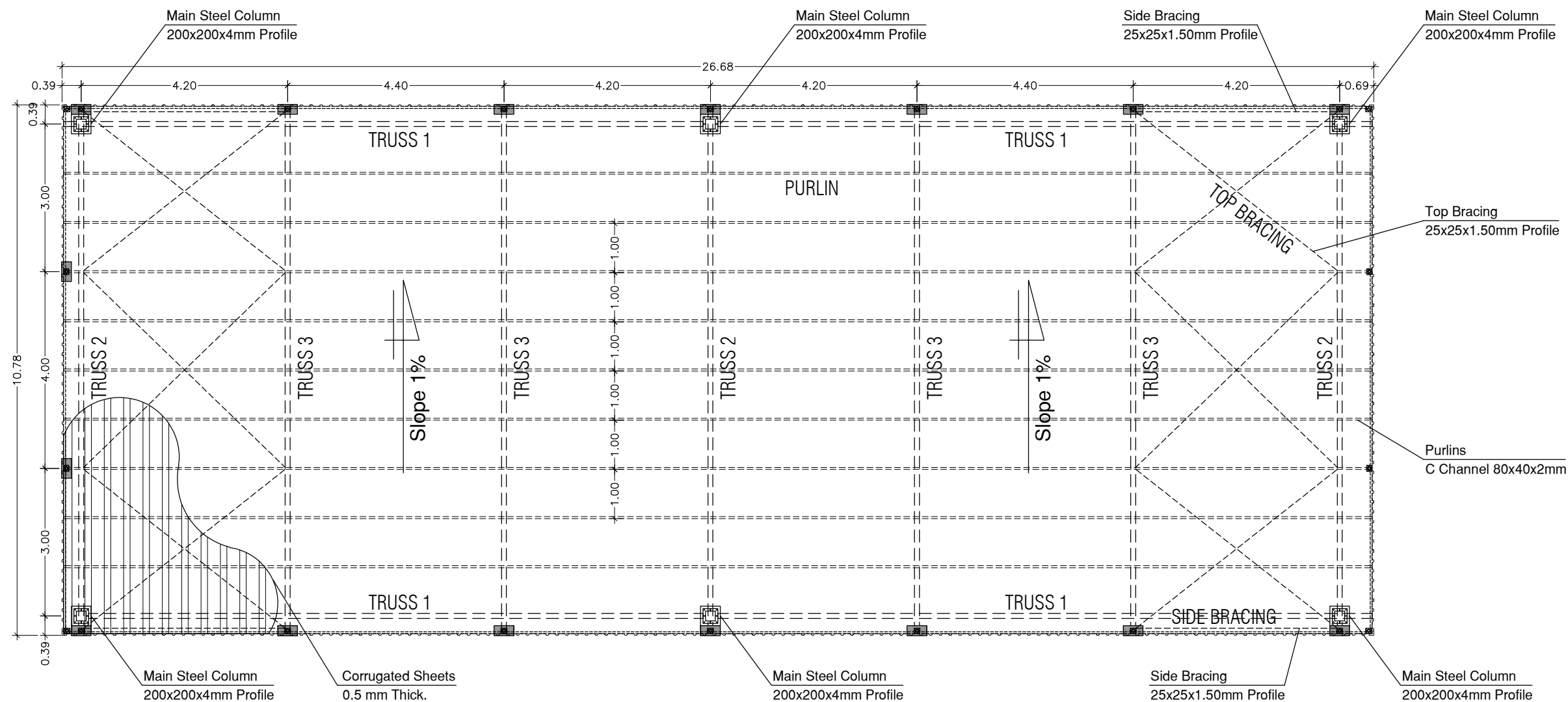
ROOF FRAMING LAYOUT SCALE 1:100
