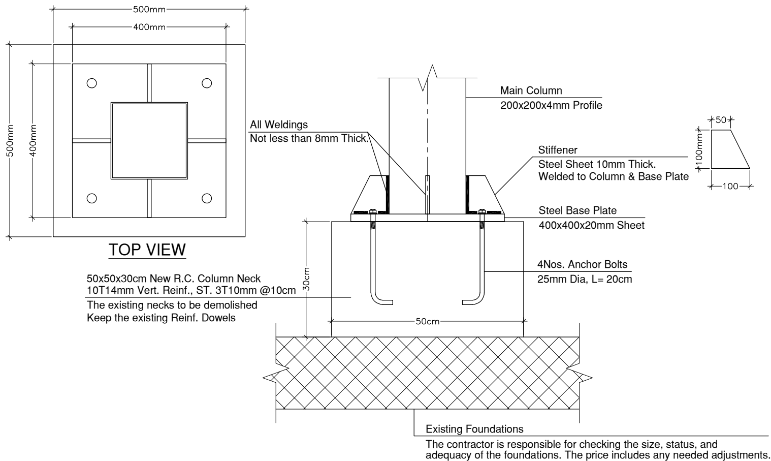
DETAIL NO. 1 SCALE 1:10
