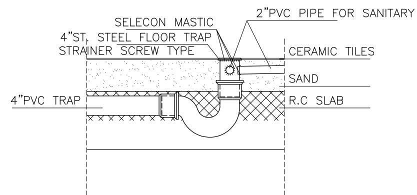
FLOOR TRAP 4/4" DETAIL
