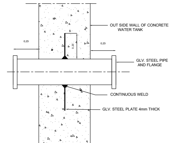
PIPE THROUGH CONCRETE WATER TANK DETAIL
