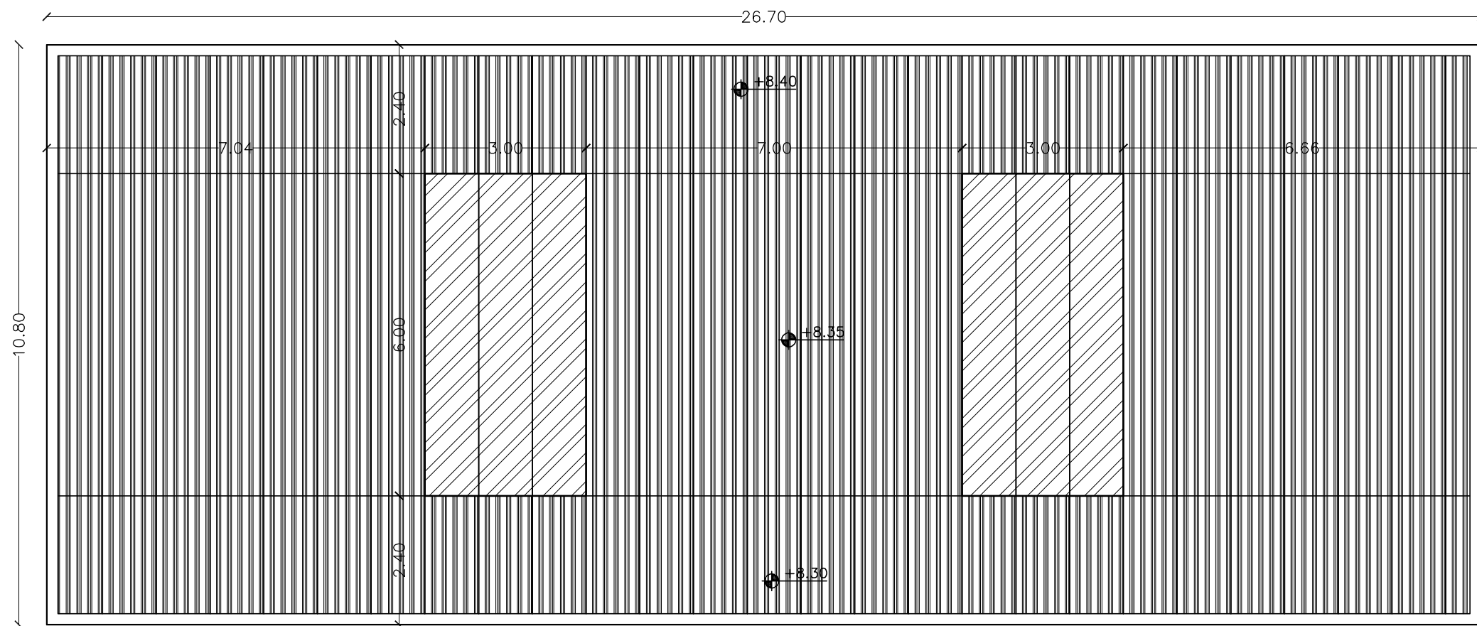
Shed Top View
