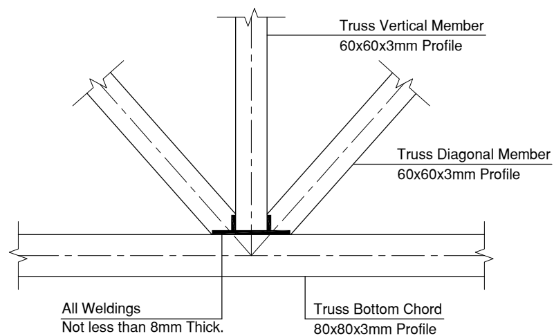
DETAIL NO. 4 SCALE 1:10
