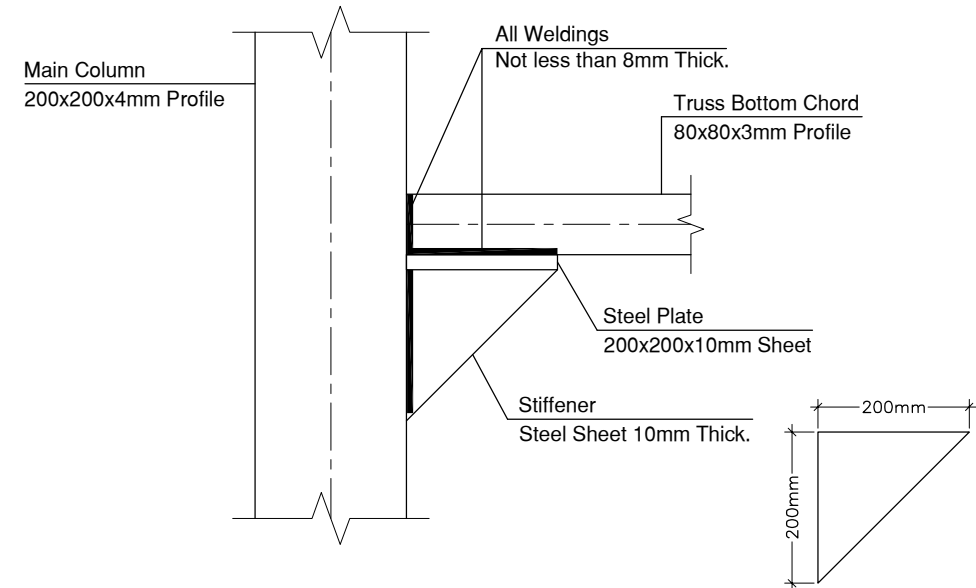
DETAIL NO. 2 SCALE 1:10
