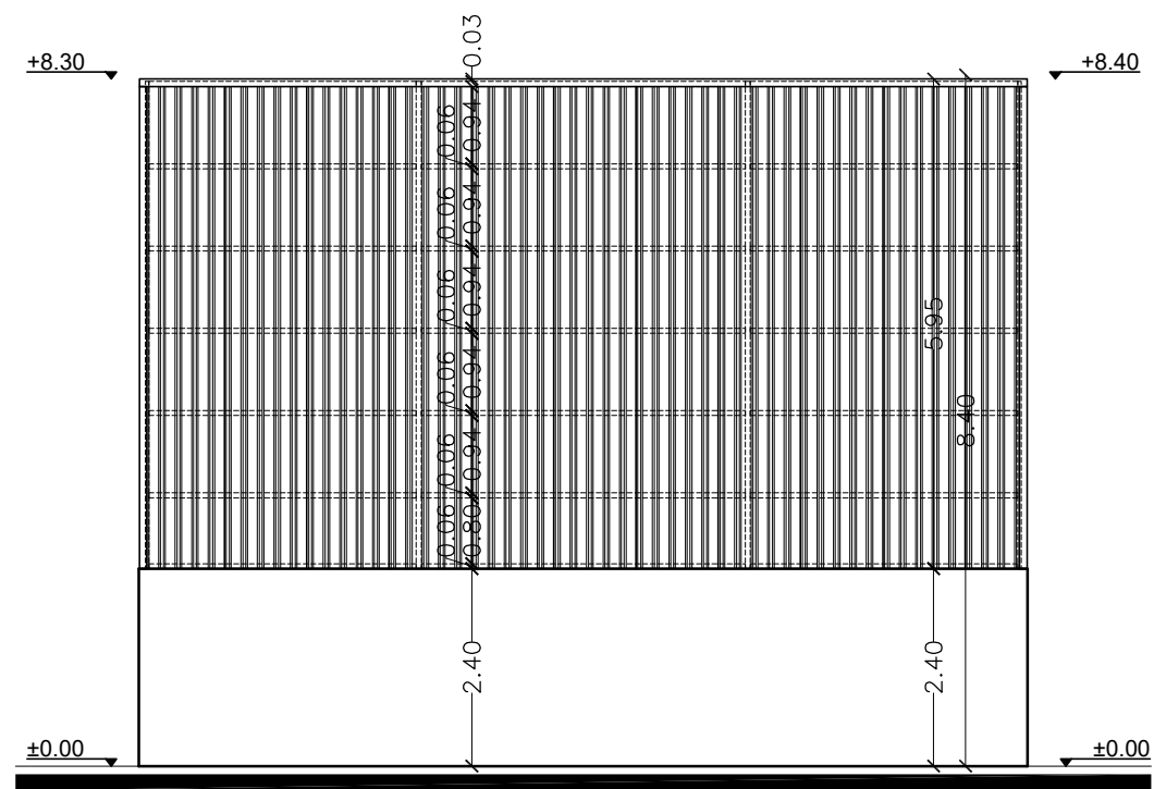
Eastern Elevation
