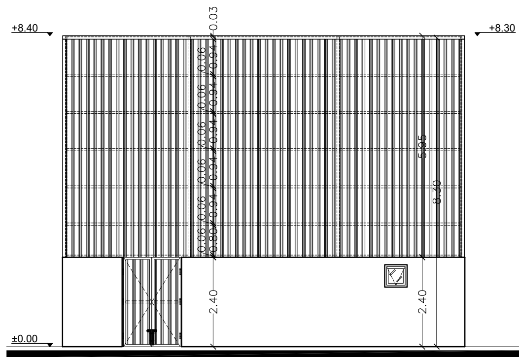
Western Elevation
