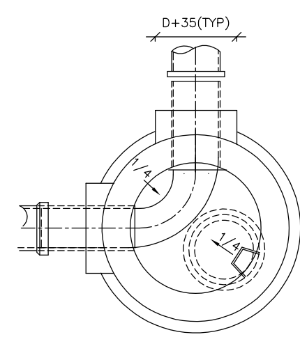
TYPICAL PLANS M.H. BENCHING NOT TO SCALE
