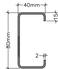
PROPERTIES OF THE PURLINS
