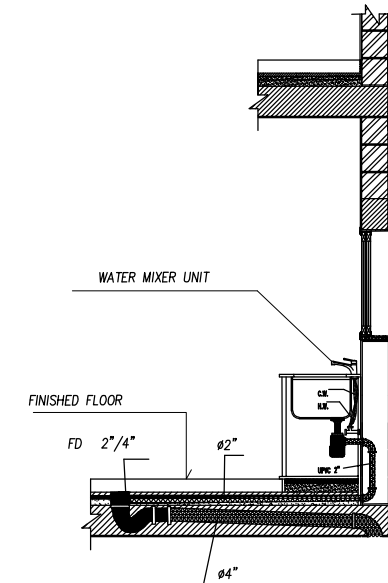
TYPICAL SINK INSTALLATION
