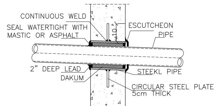
PIPE SLEEVE DETAIL
