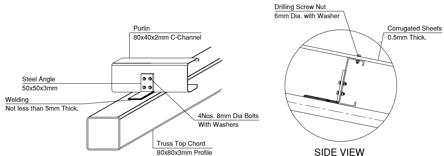
DETAIL FOR PURLINS CONNECTION NOT TO SCALE
