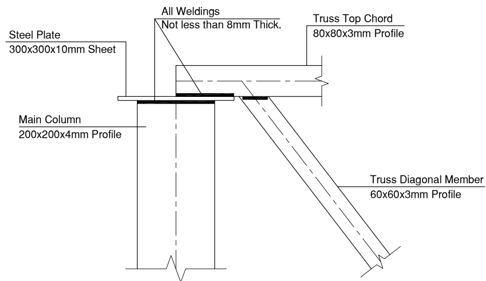
DETAIL NO. 3 SCALE 1:10
