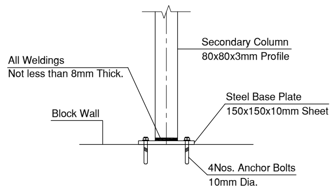
DETAIL NO. 5 SCALE 1:10
