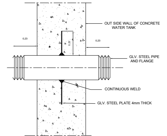
PIPE THROUGH CONCRETE WATER TANK DETAIL
