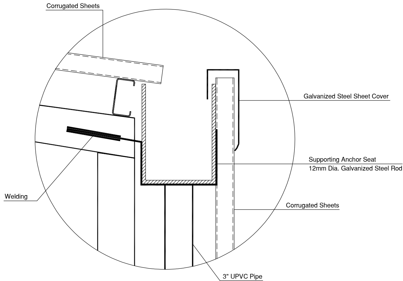
GENERAL DETAILS FOR RAIN WATER GUTTER NOT TO SCALE
