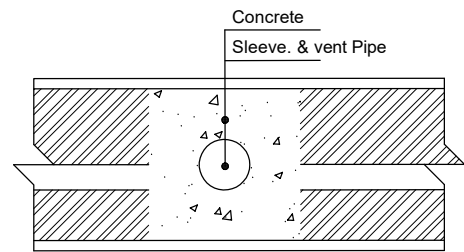
UPVC PIPES IN THE WALLS
