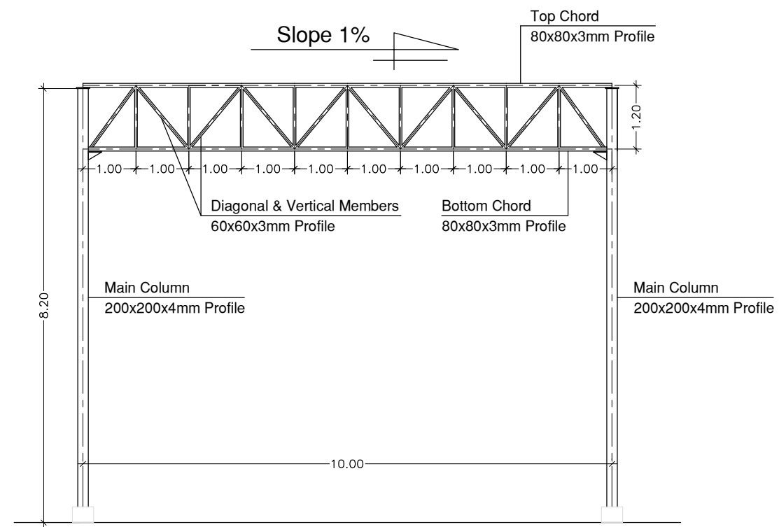
TRUSS 2 SECTION SCALE 1:100
