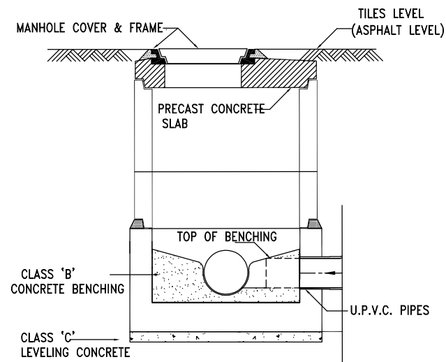
TYPICAL MANHOLE SECTION NOT TO SCALE
