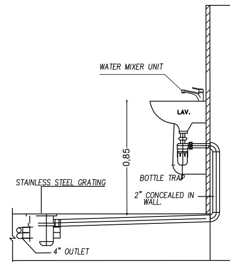
TYPICAL LAVATORY INSTALLATION
