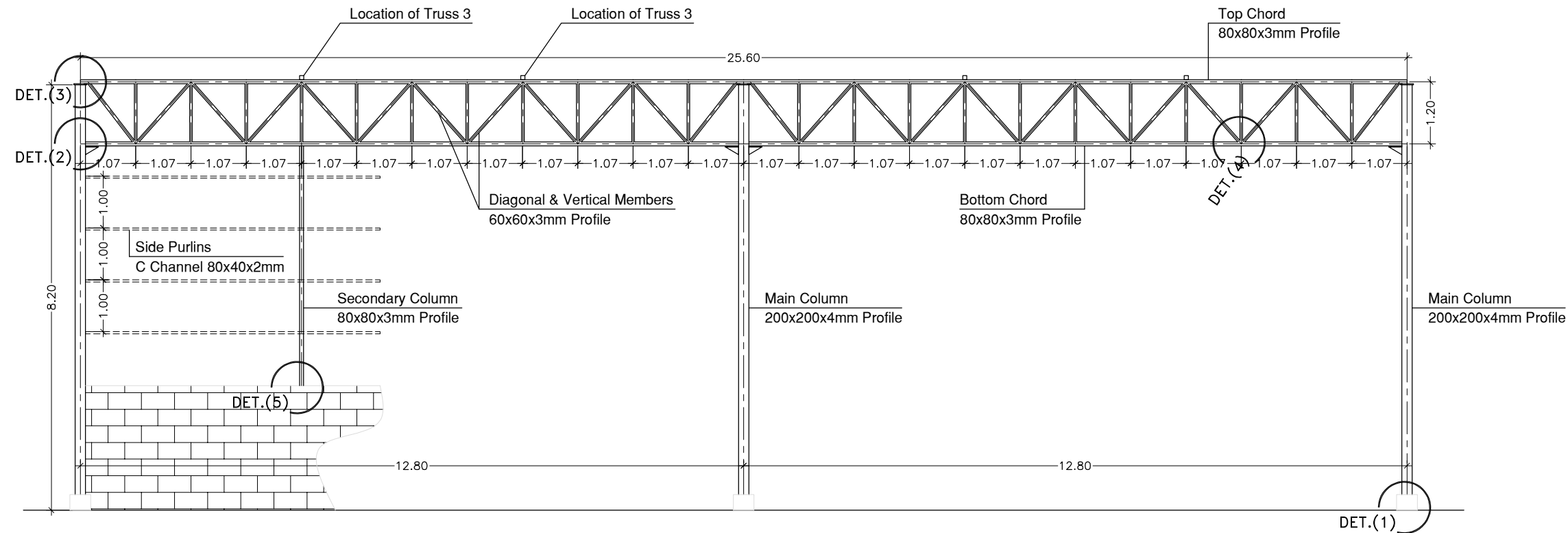
TRUSS 1 SECTION SCALE 1:100
