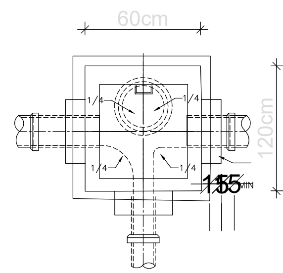
TYPICAL PLANS C.H. BENCHING NOT TO SCALE
