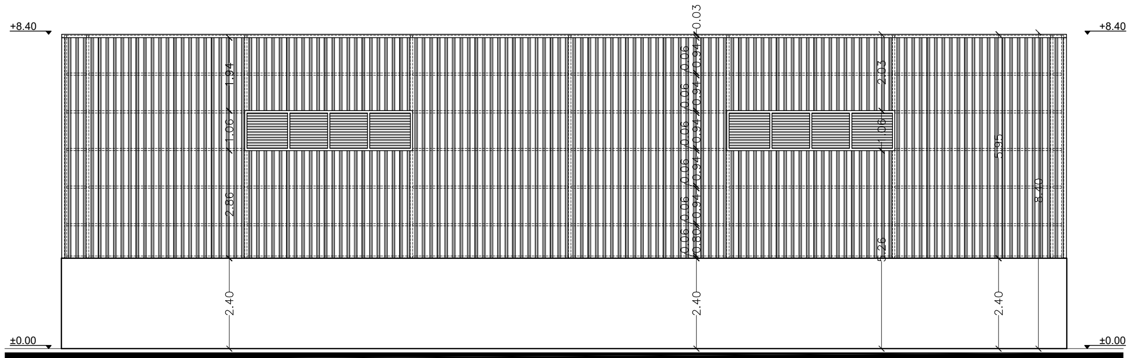
Northern Elevation
