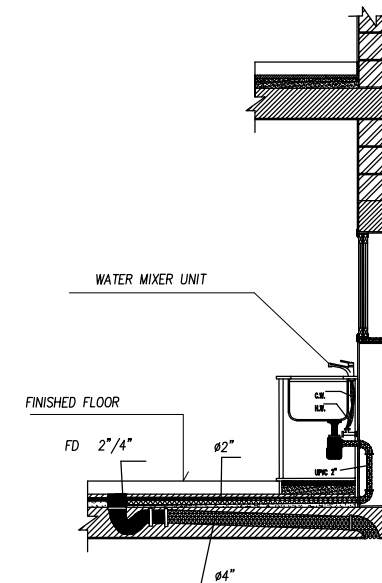
TYPICAL SINK INSTALLATION
