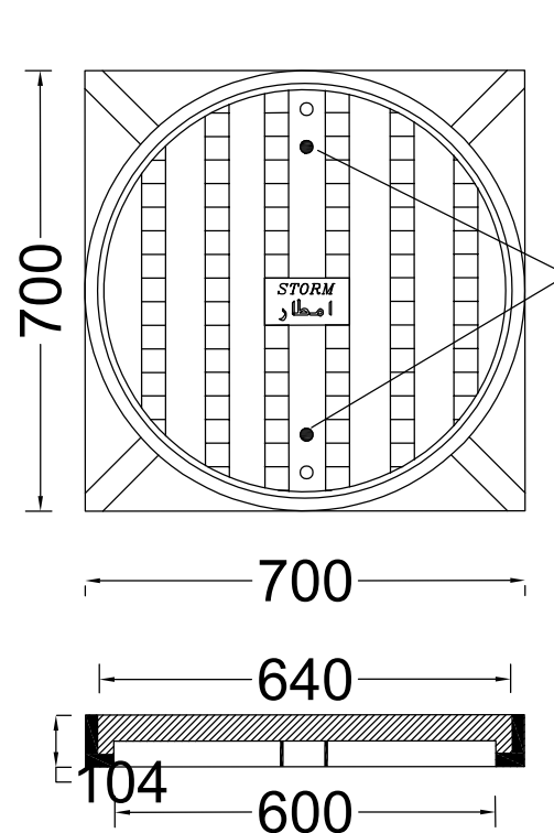
Cast Iron Lockable Cover
