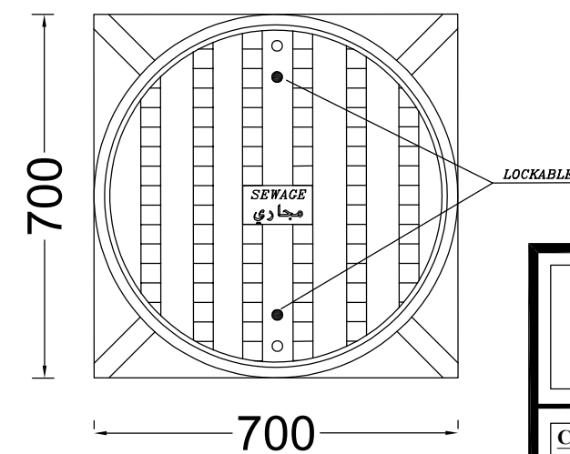
Cast Iron Lockable Cover
