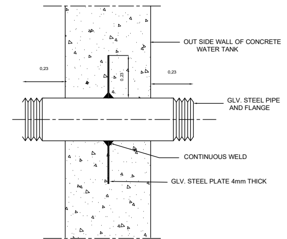
PIPE THROUGH CONCRETE WATER TANK DETAIL
