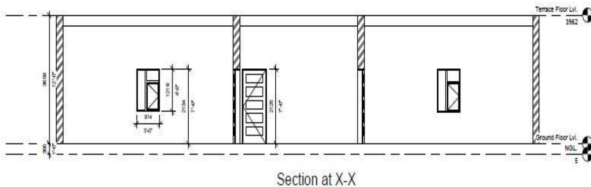
Figure 2: Section drawing Chotagaghra community centre:
