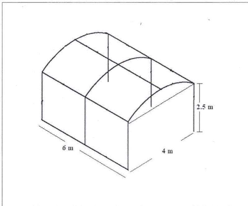
Construction of Greenhouse (Solar Dryer) for AD Programme Areas in Loilen Township
