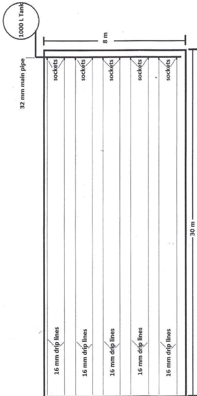
Drip Irrigation System for 30m length and 8m greenhouse
