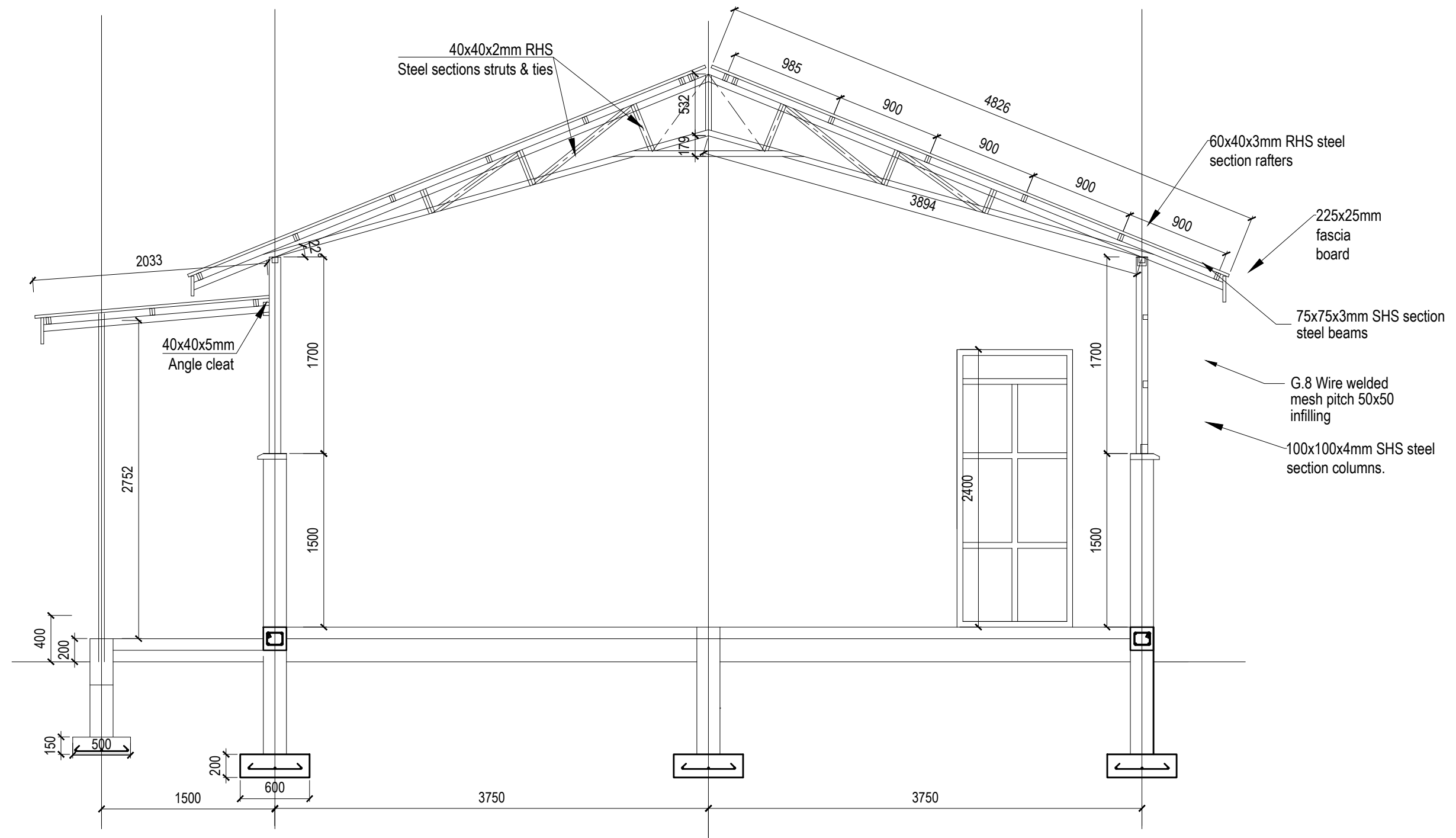
SECTIONAL ELEVATION
