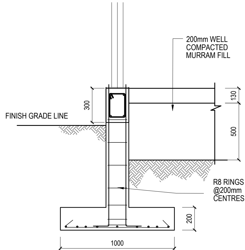
PAD FOOTING SECTION
